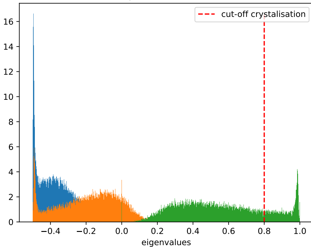
Distribution of eigenvalues at T = 0.575 , \dot{T} = 10^{-7}
