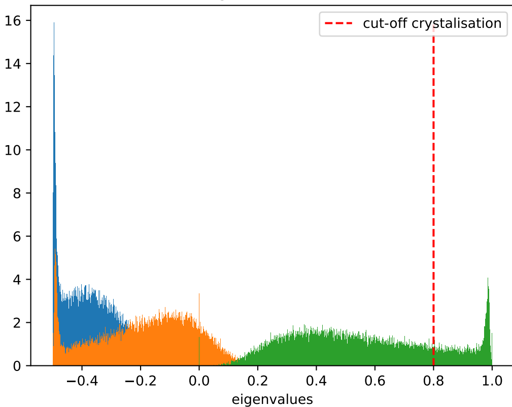
Distribution of eigenvalues at T = 0.6 , \dot{T} = 10^{-7}
