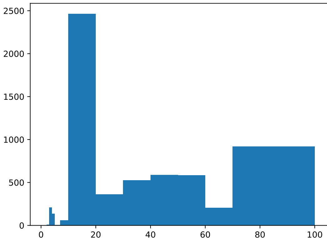
Crystalline domain size distribution, PVA-100, time 12000000, \phi = 0.372
