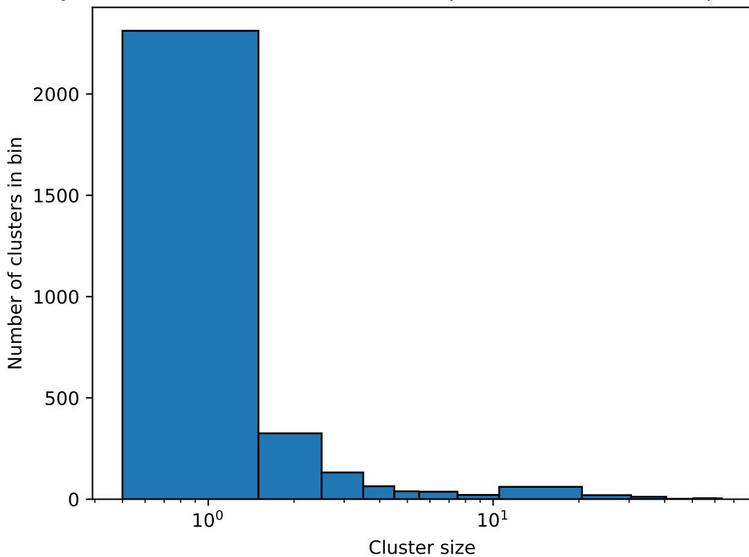
Crystalline domain size distribution, quench 10^{-3} , PVA-100, \phi = 0.186
