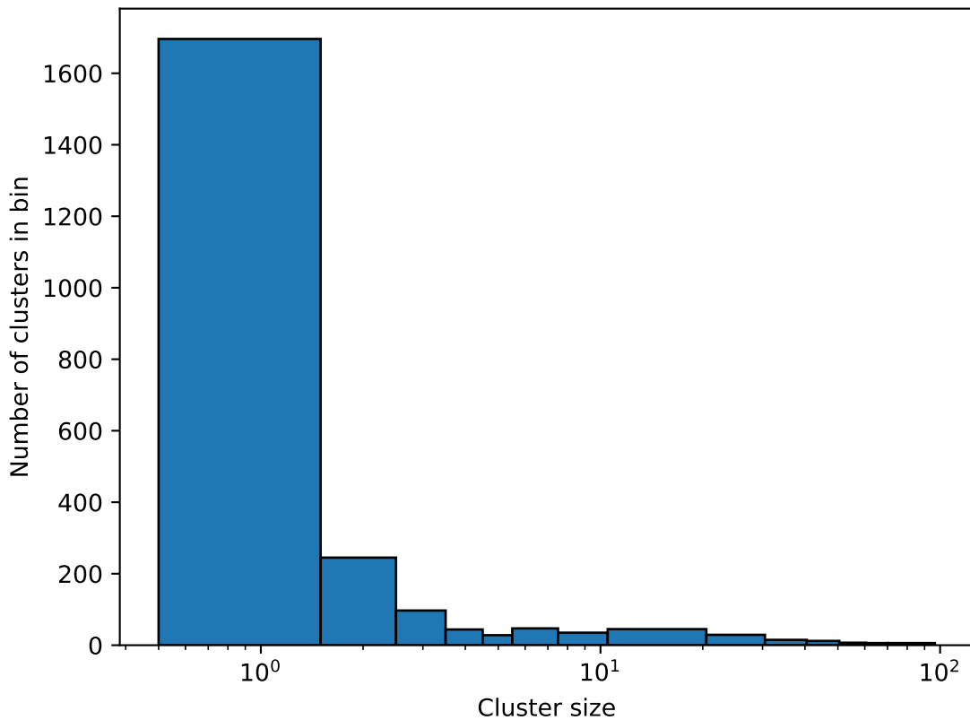
Crystalline domain size distribution, quench 10^{-3} , PVA-100, \phi = 0.199
