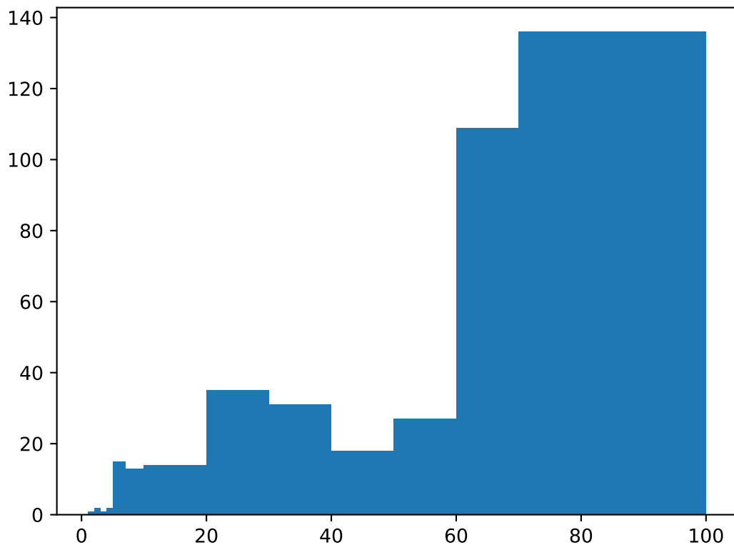
Crystalline domain size distribution, PVA-100, time 5000000, \phi = 0.183
