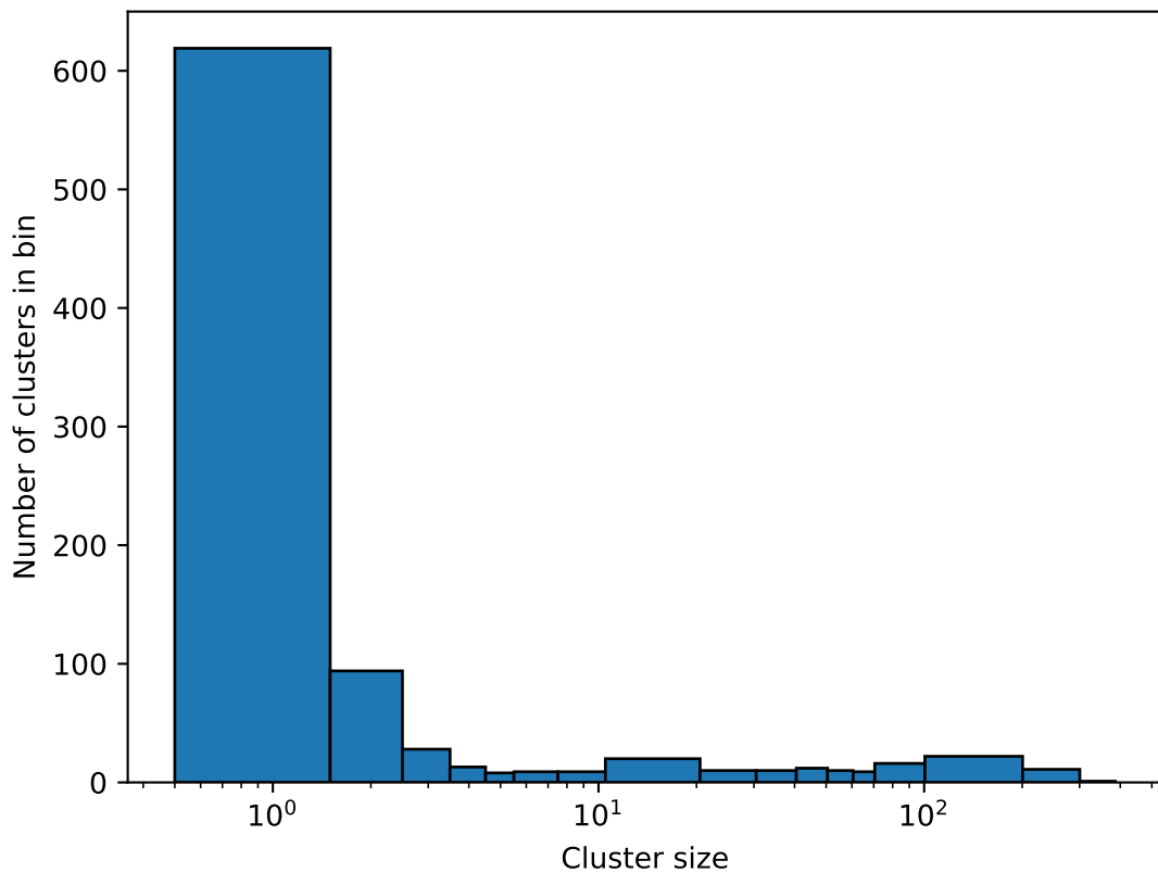
Crystalline domain size distribution, PVA-1000, \phi = 0.313
