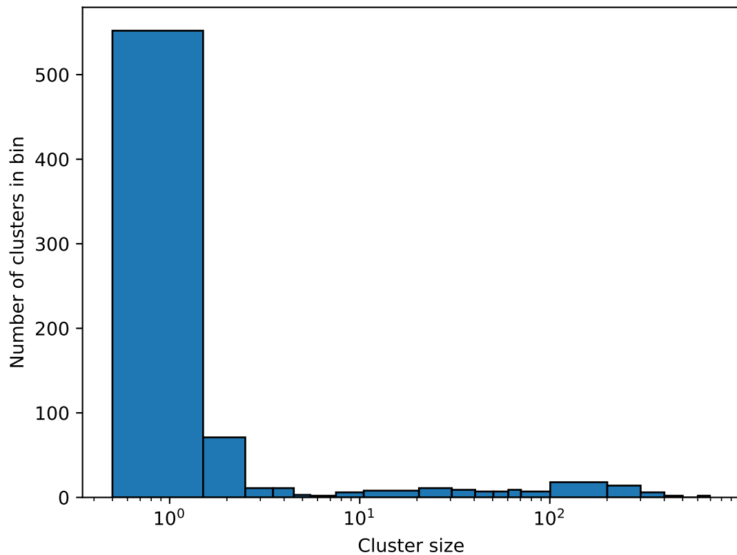
Crystalline domain size distribution, PVA-1000, \phi = 0.377
