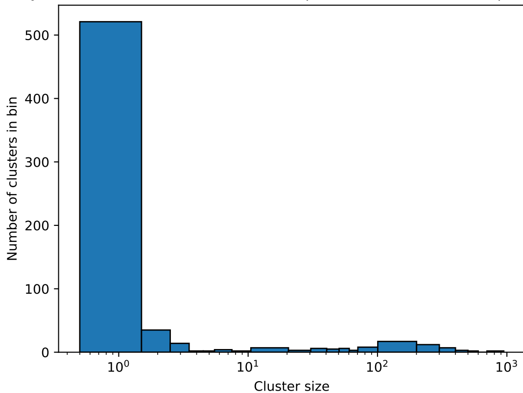
Crystalline domain size distribution, quench 10^{-3} , PVA-1000, \phi = 0.416
