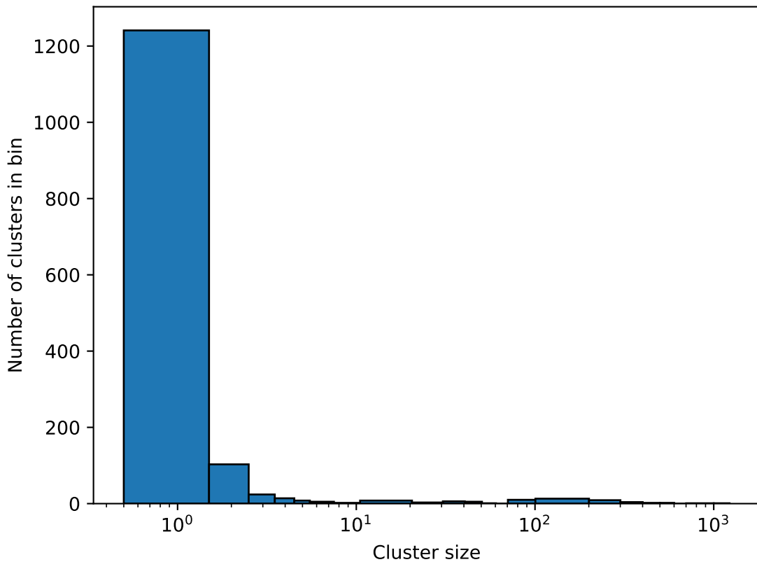
Crystalline domain size distribution, quench 10^{-3} , PVA-50, \phi = 0.351
