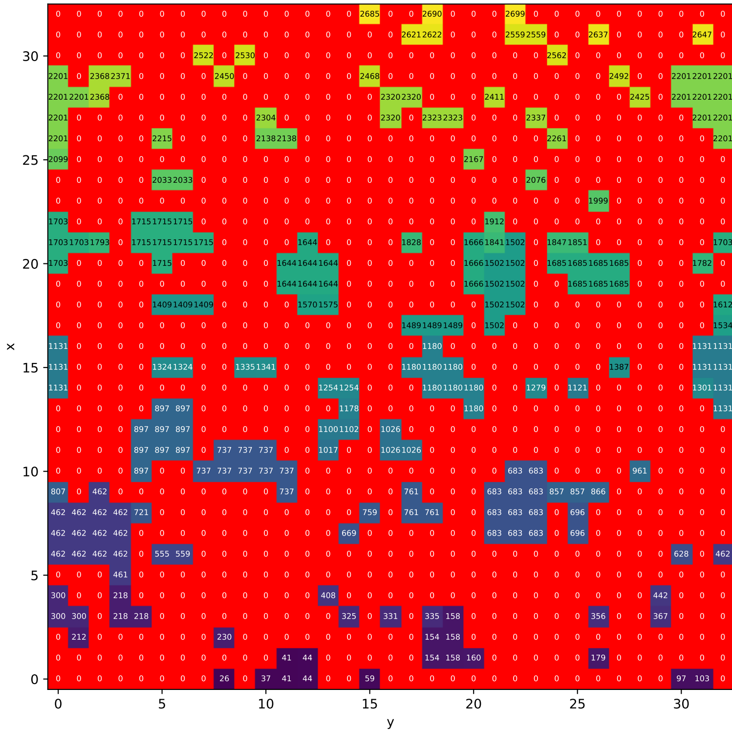
Cluster labels, PVA-100, T = 0.5 , T_{\text{dot}} = 10^{**}(-5) , T_{\text{init}} = 1.0 , z = 28
