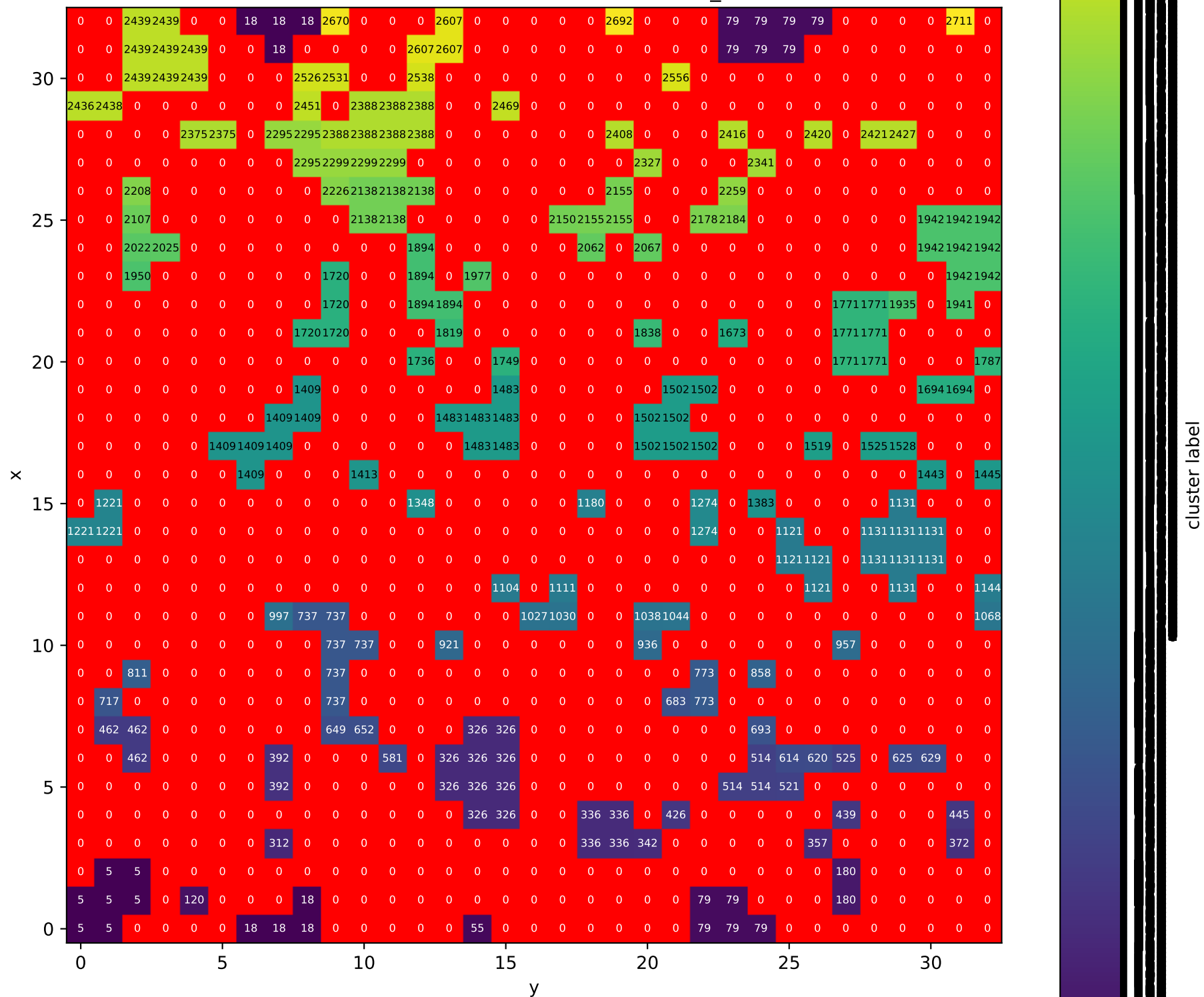
Cluster labels, PVA-100, T = 0.5, Tdot = 10**(-5), T_init = 1.0, z = 30
