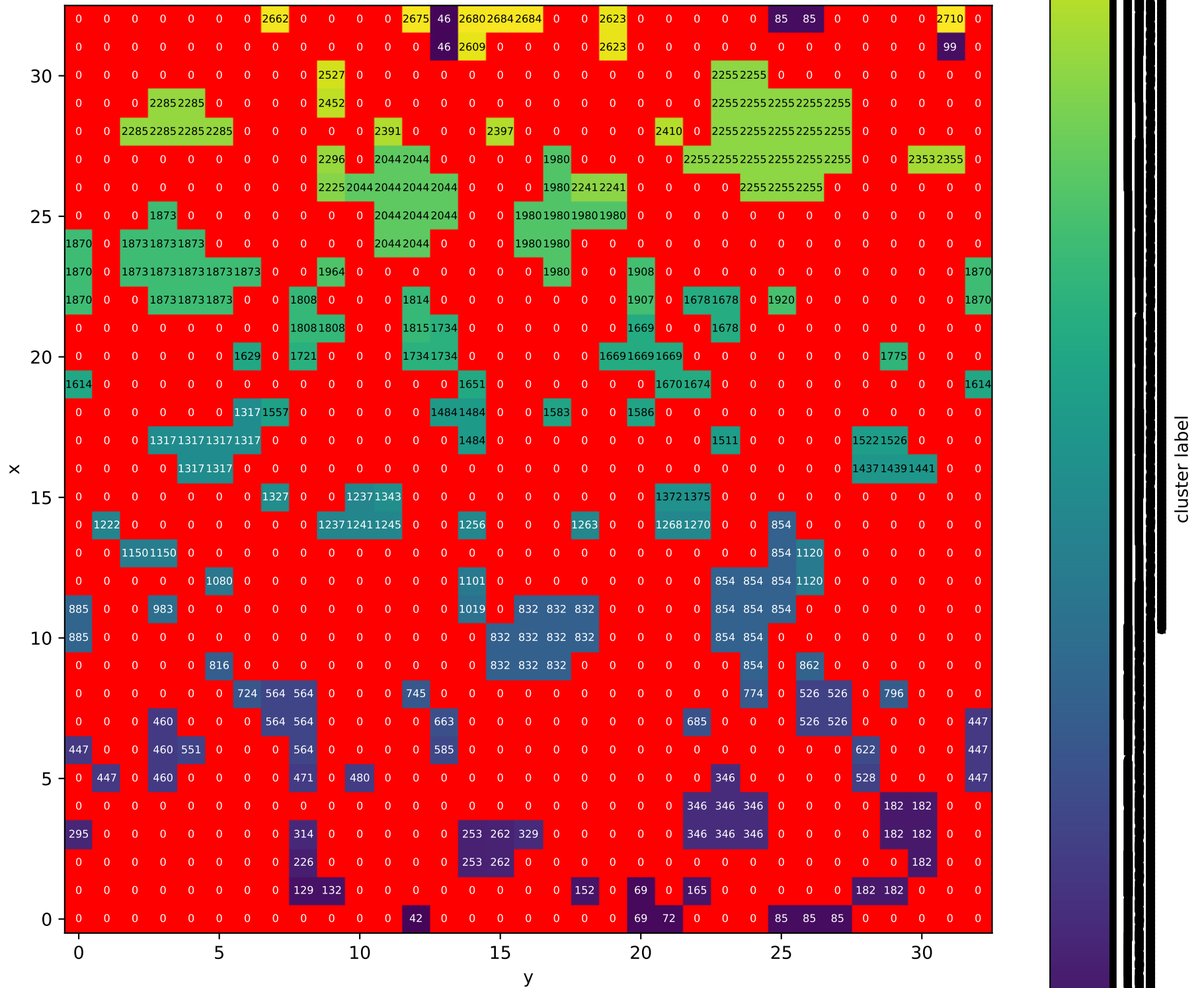
Cluster labels, PVA-100, T = 0.5 , T_{\text{dot}} = 10^{**}(-5) , T_{\text{init}} = 1.0 , z = 6
