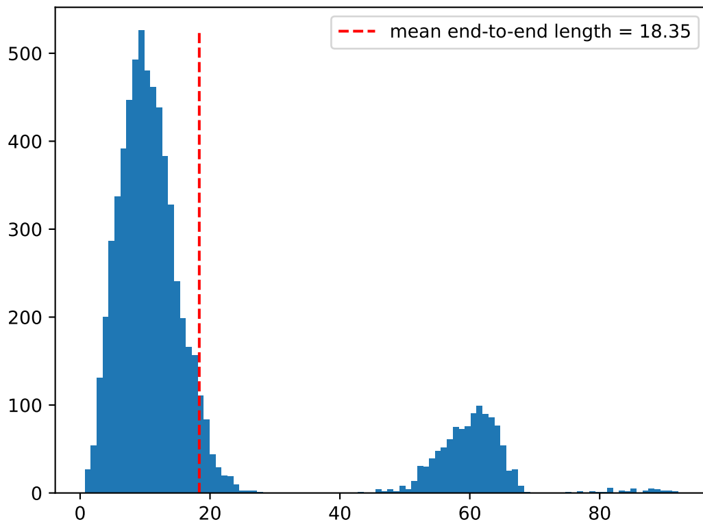
Distribution of end-to-end distance
