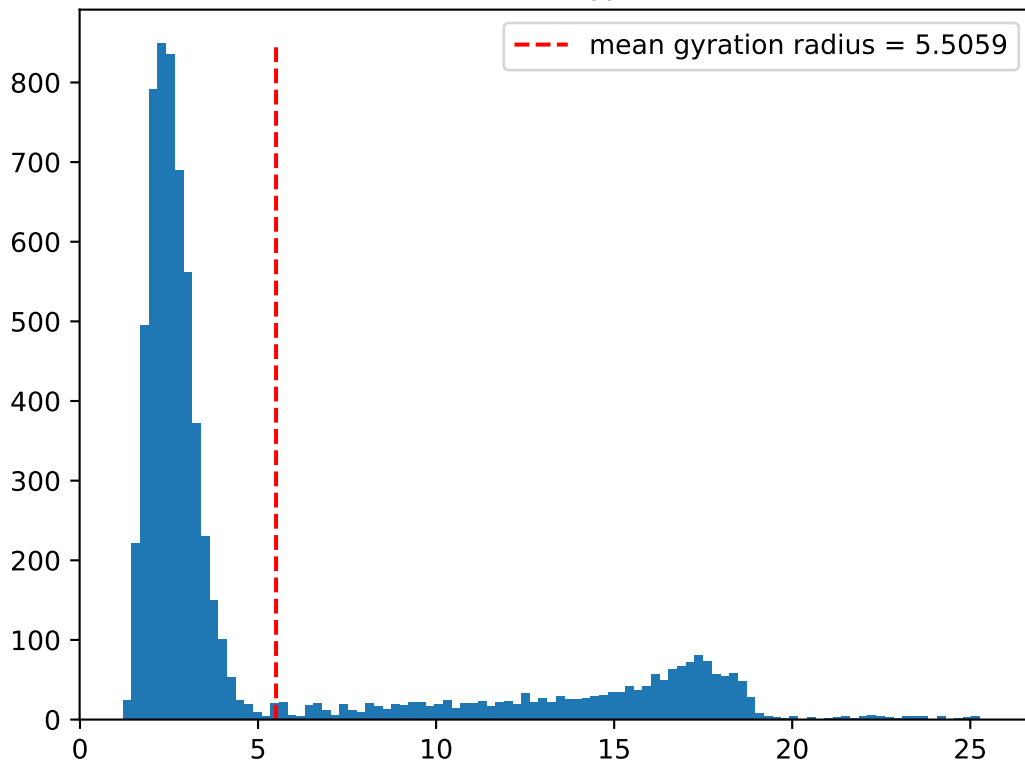
Distribution of the gyration radius
