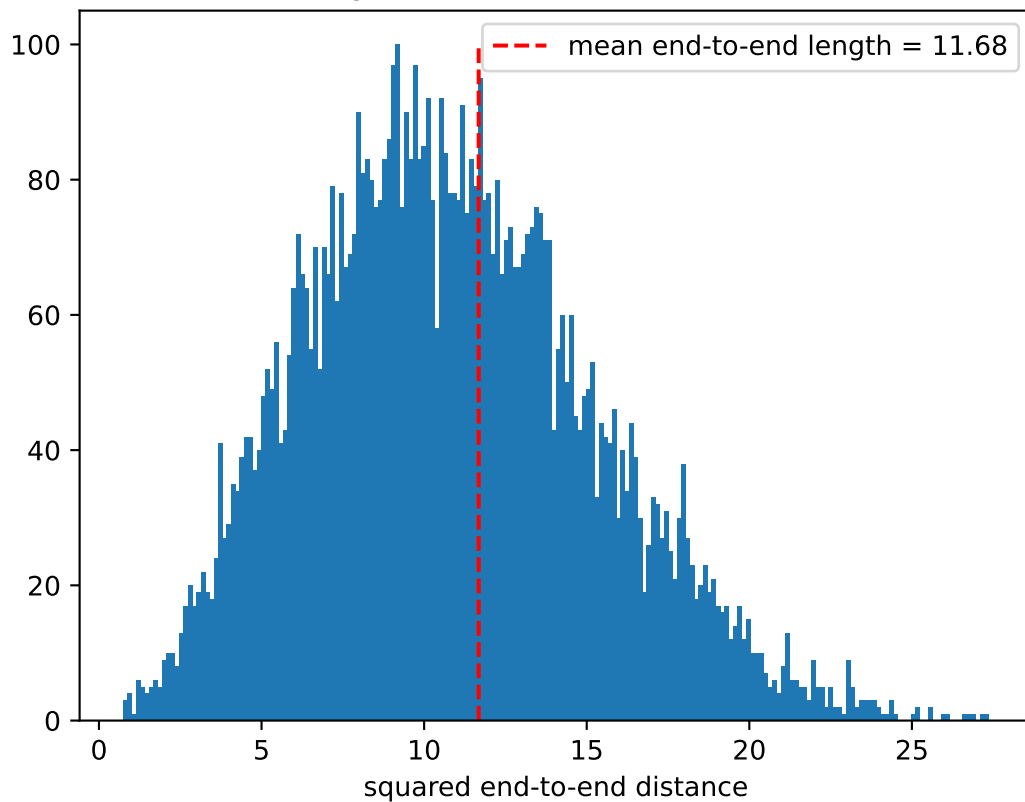
End-to-end length distribution, PVA-100, \dot{T} = 10^{-3} , T = 1
