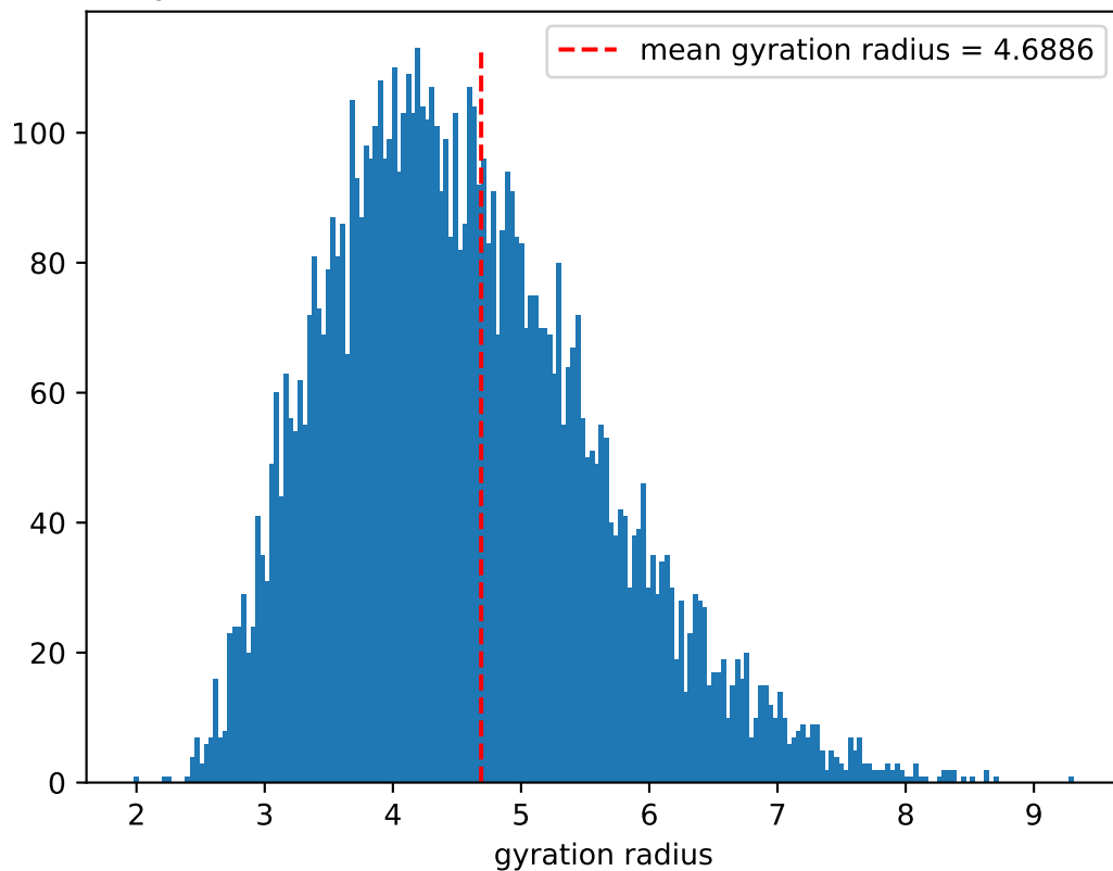
Gyration radius distribution, PVA-100, \dot{T} = 10^{-3} , T = 0.5
