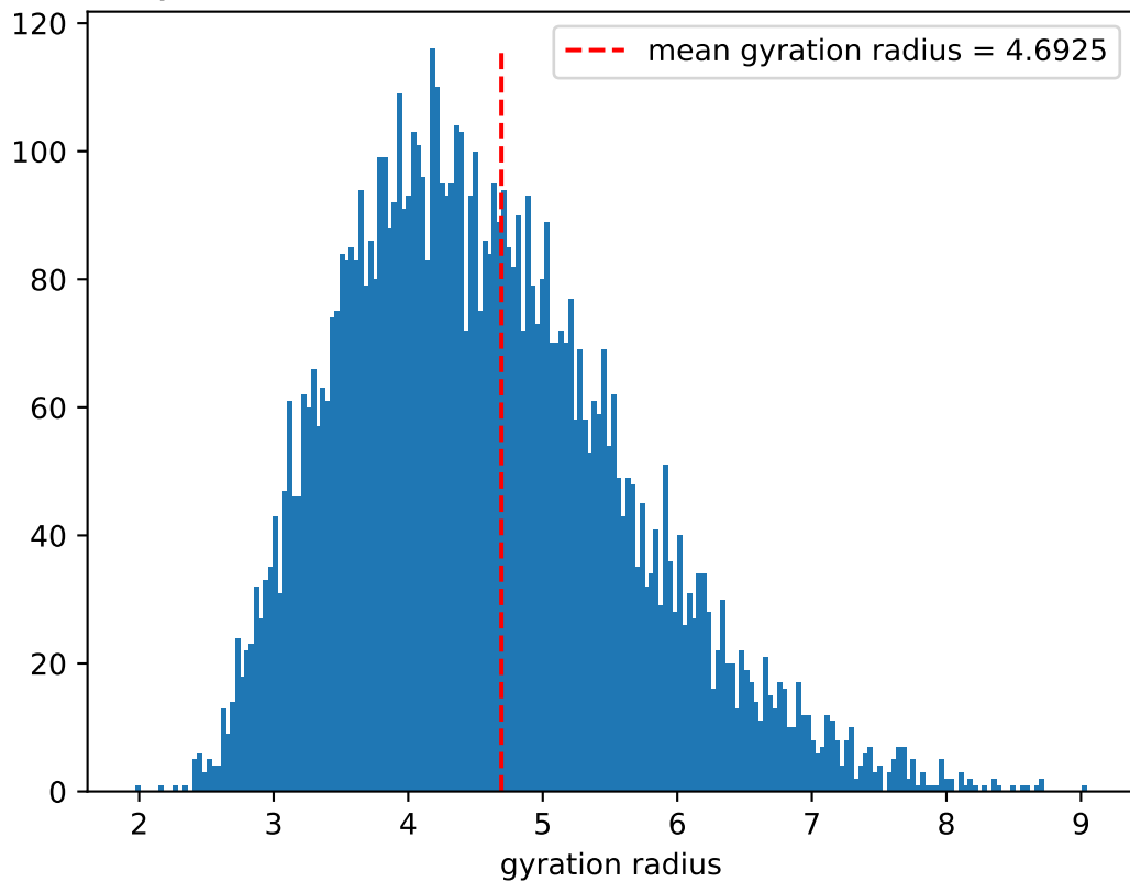
Gyration radius distribution, PVA-100, \dot{T} = 10^{-3} , T = 0.7
