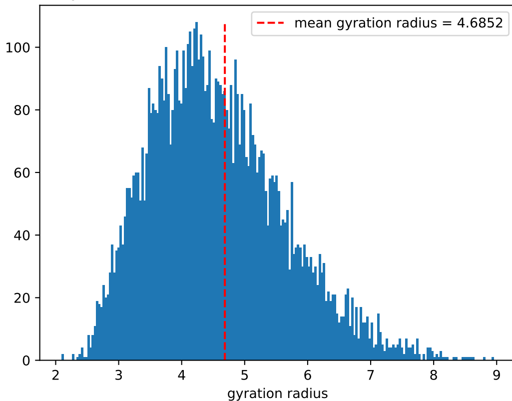
Gyration radius distribution, PVA-100, \dot{T} = 10^{-3} , T = 0.8
