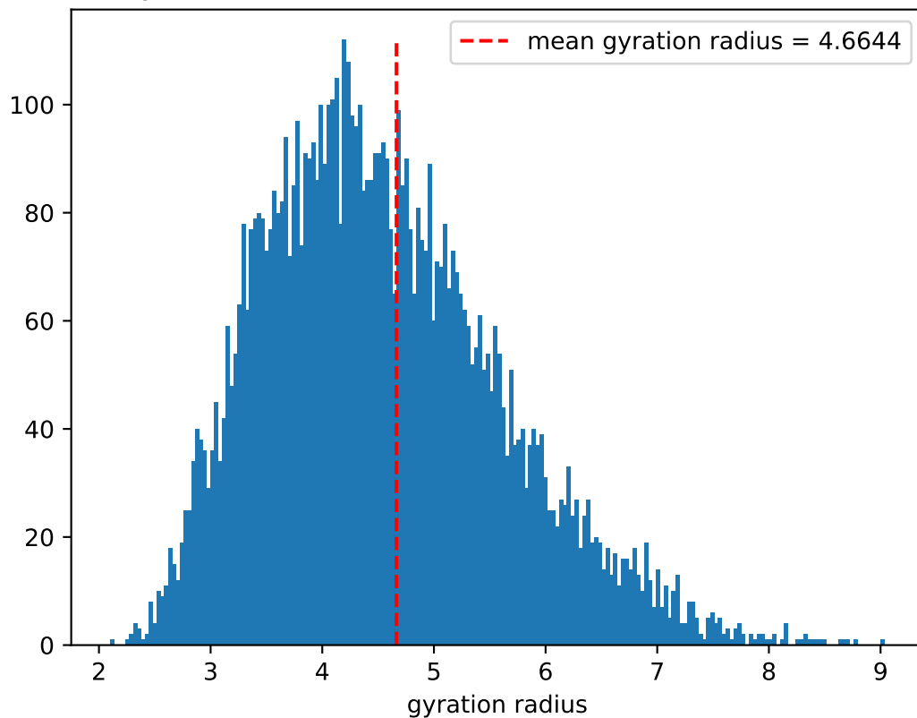
Gyration radius distribution, PVA-100, \dot{\gamma} = 10^{-3} , T = 1
