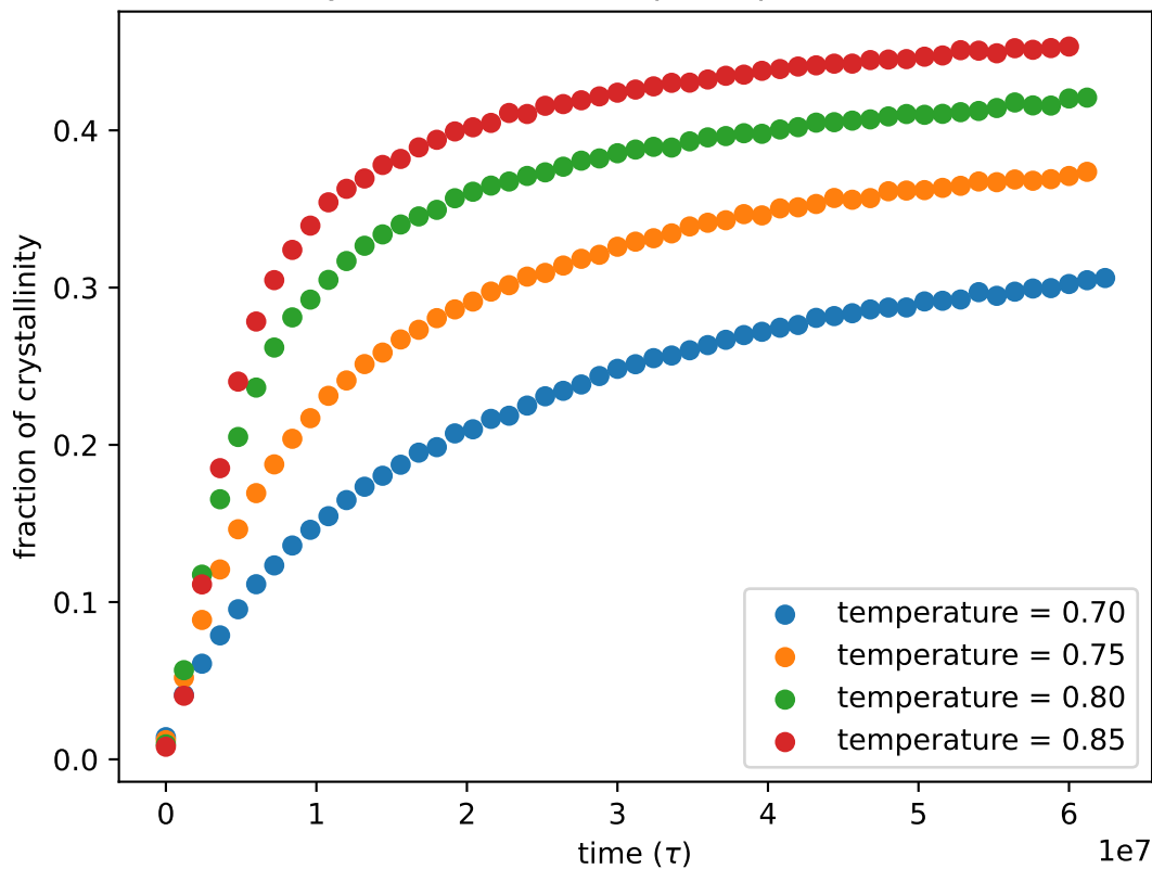
PVA-100 crystallisation after quick quench at \dot{T} = 10^{-3} \tau^{-1}
