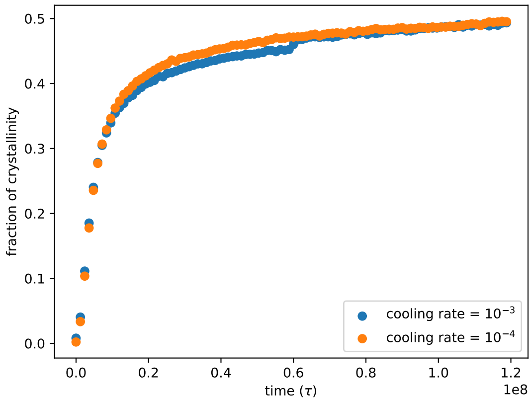
PVA-100 crystallisation after quick quench at T = 0.85
