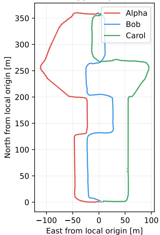
Square 1: distributed PCM + CBS Dotted: supplied position GT
