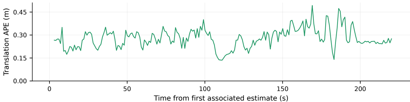
Carol | evo APE RMSE 0.29 m
