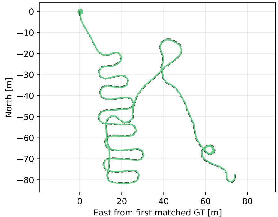
Carol: raw odometry evo ATE 0.255 m
