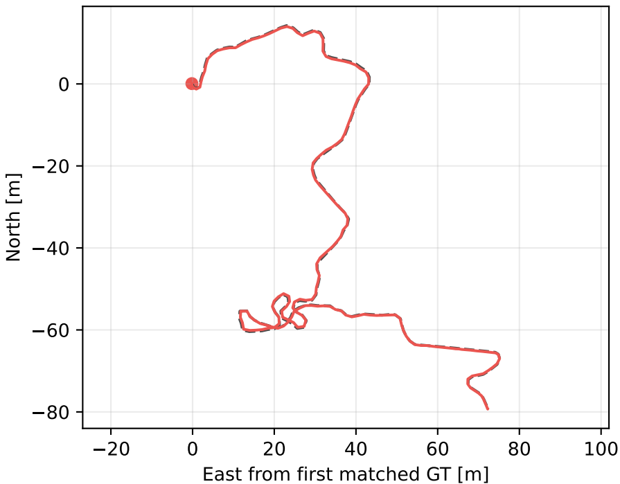
Alpha: raw odometry evo ATE 0.194 m
