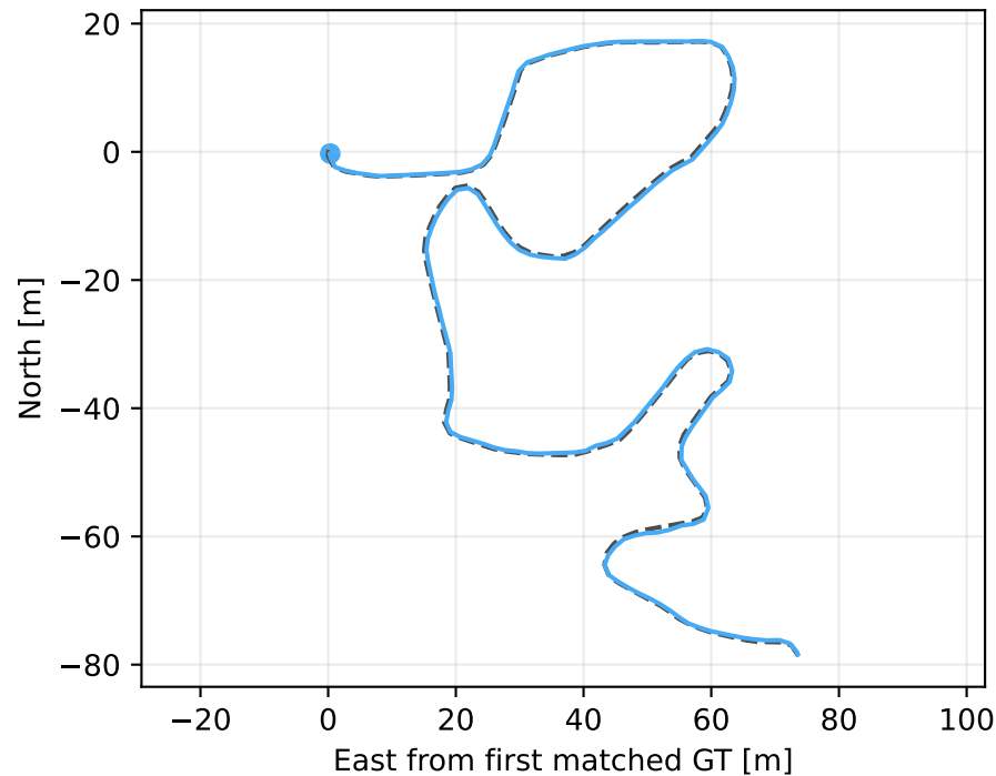
Bob: raw odometry evo ATE 0.330 m
