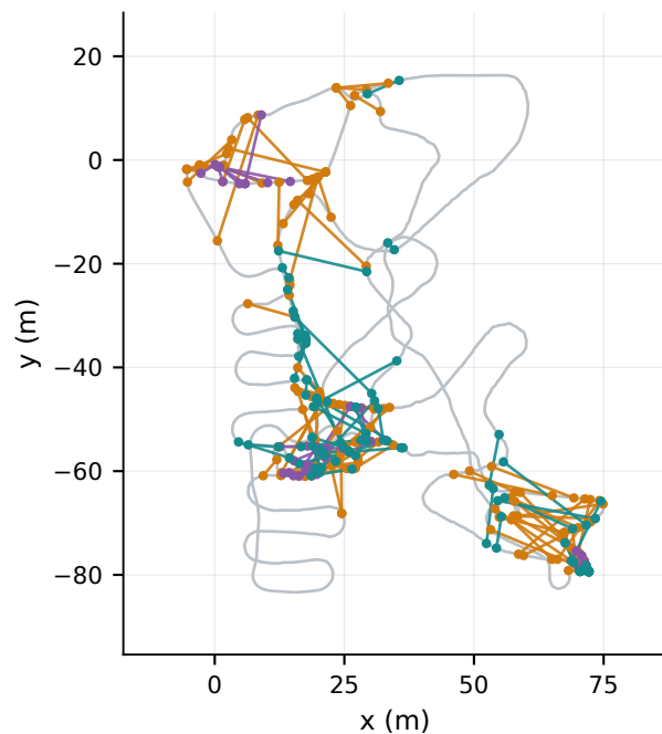
(b) Verified loop closures
