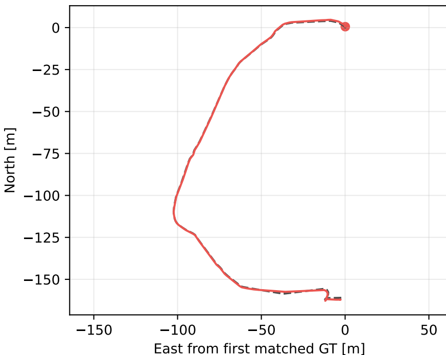
Alpha: raw odometry evo ATE 0.544 m
