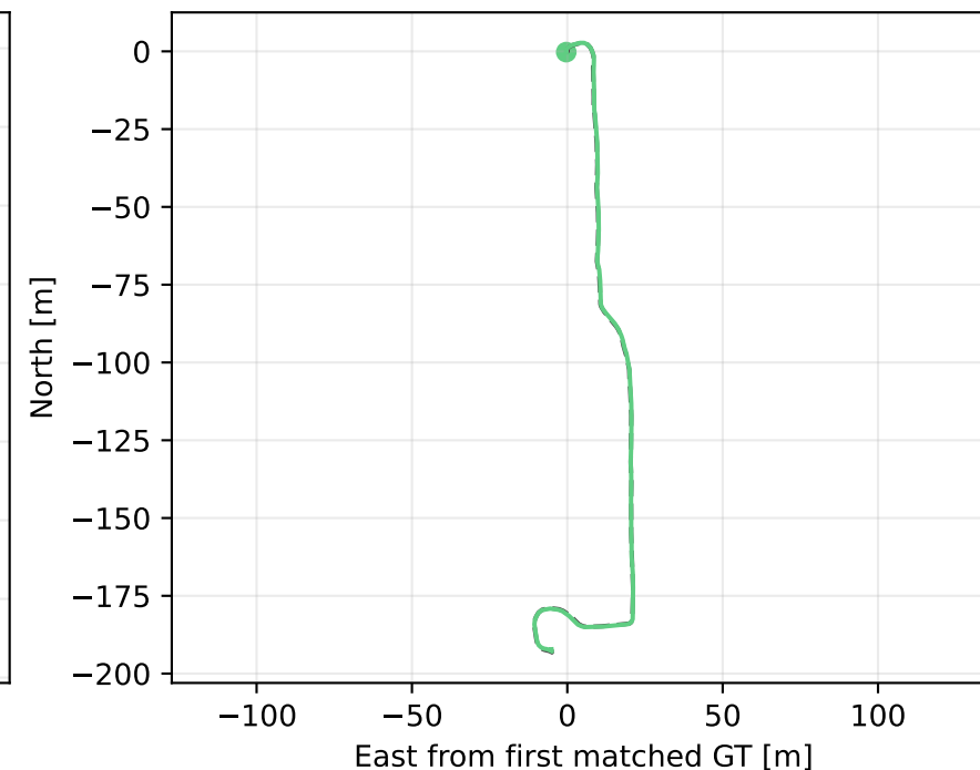
Carol: raw odometry evo ATE 0.218 m
