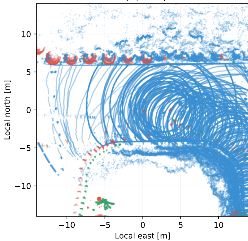
3. End overlap | CBS pose factors
