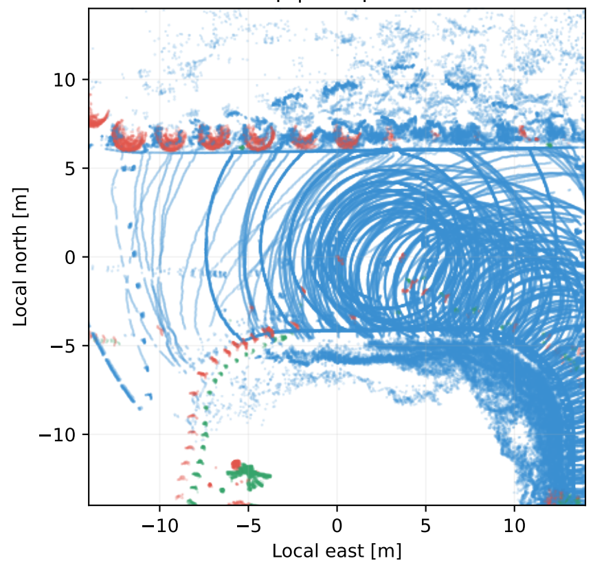
3. End overlap | CBS pose + live GICP
