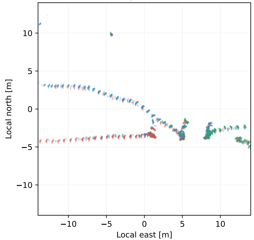
2. Junction overlap | CBS pose + live GICP
