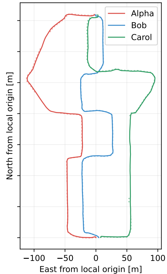
PCM + CBS pose and live GICP factors
