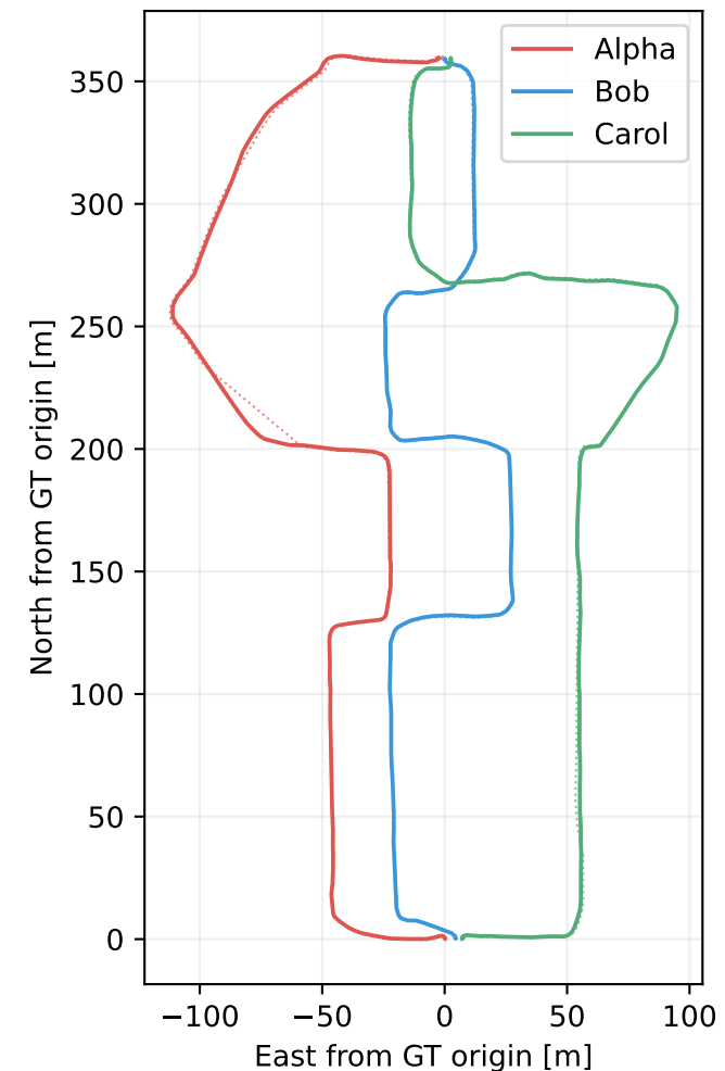
Ellipsoid-surface BEVs → centralized PGO Combined ATE 1.1408 m
