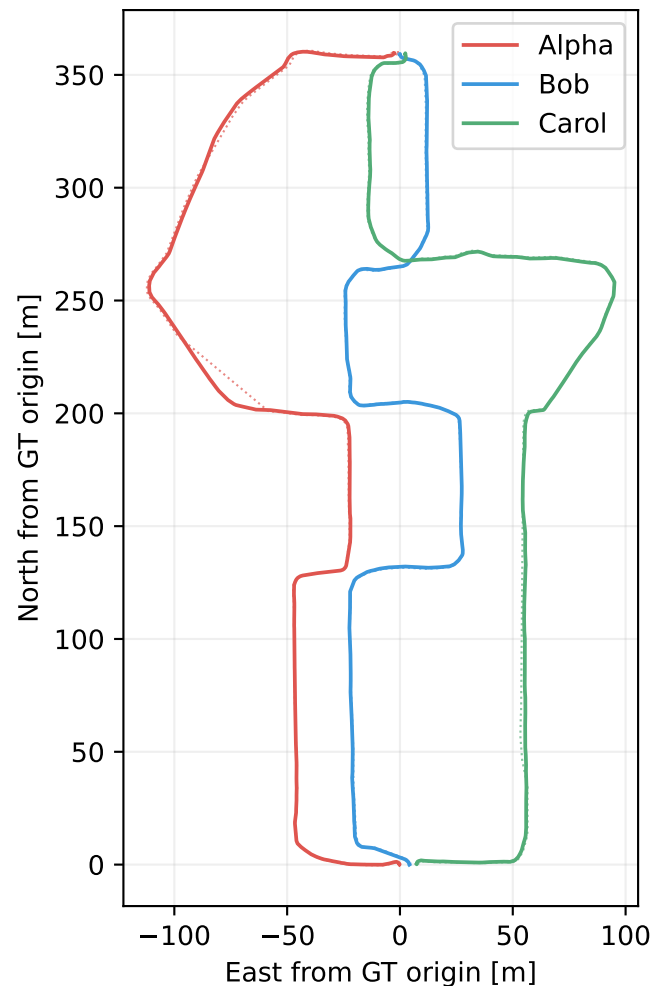
Raw-cloud BEVs → centralized PGO Combined ATE 1.1457 m
