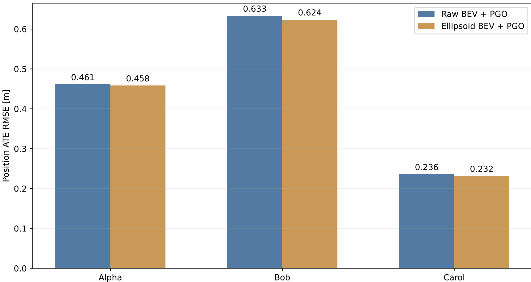
Individual robot errors after each graph's component-wide evo alignment
