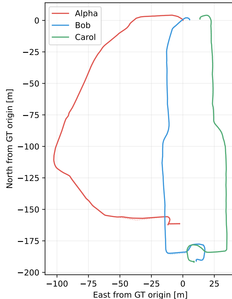
Raw-cloud BEVs → centralized PGO Combined ATE 0.4703 m
