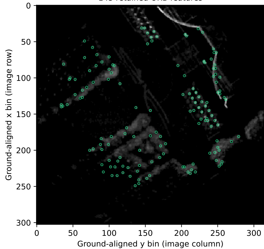
Bob 31 — Native ellipsoid surfaces (spatial map) 143 retained ORB features
