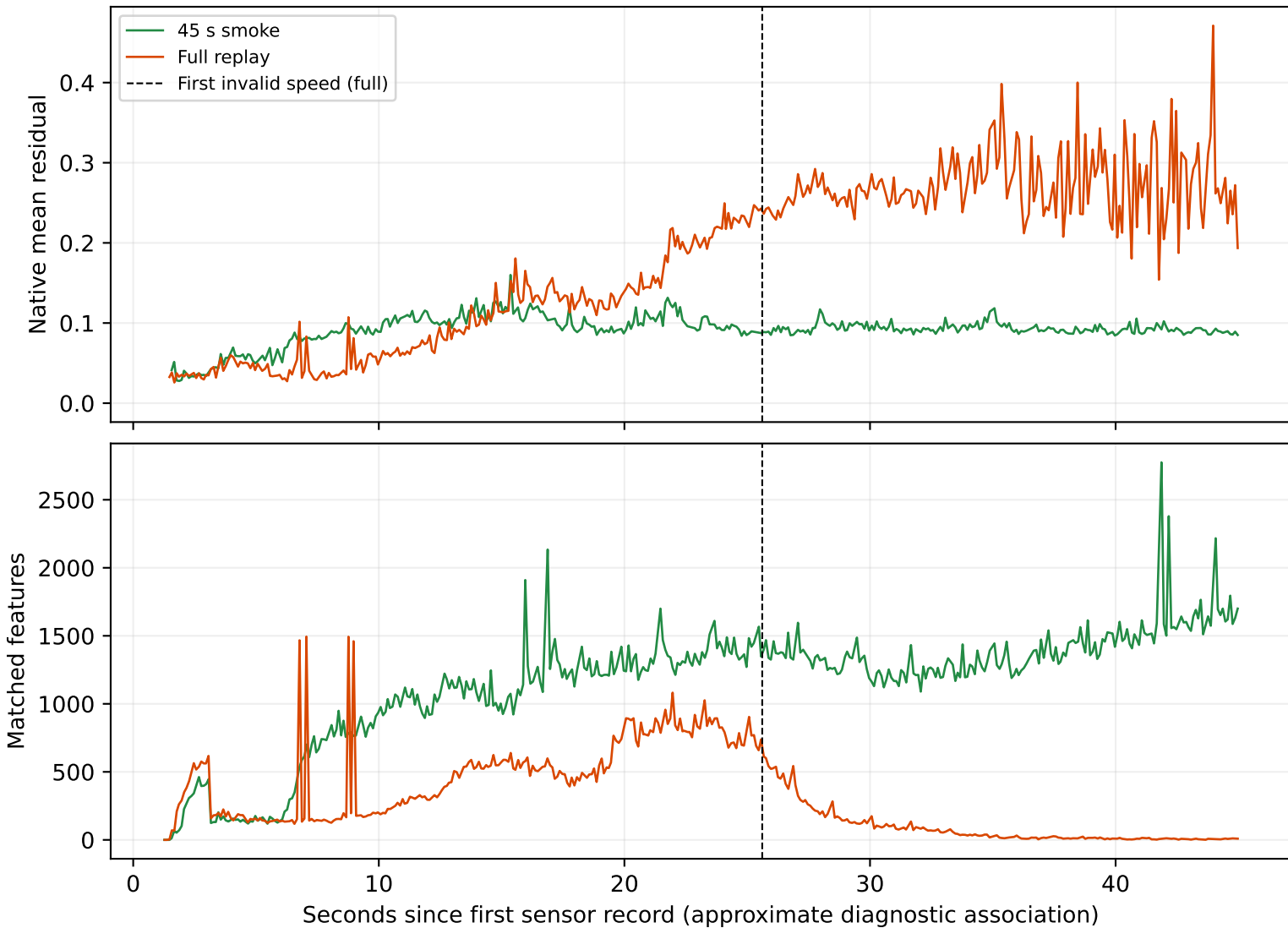
GRACO ground-01: different outcomes on the same input prefix
