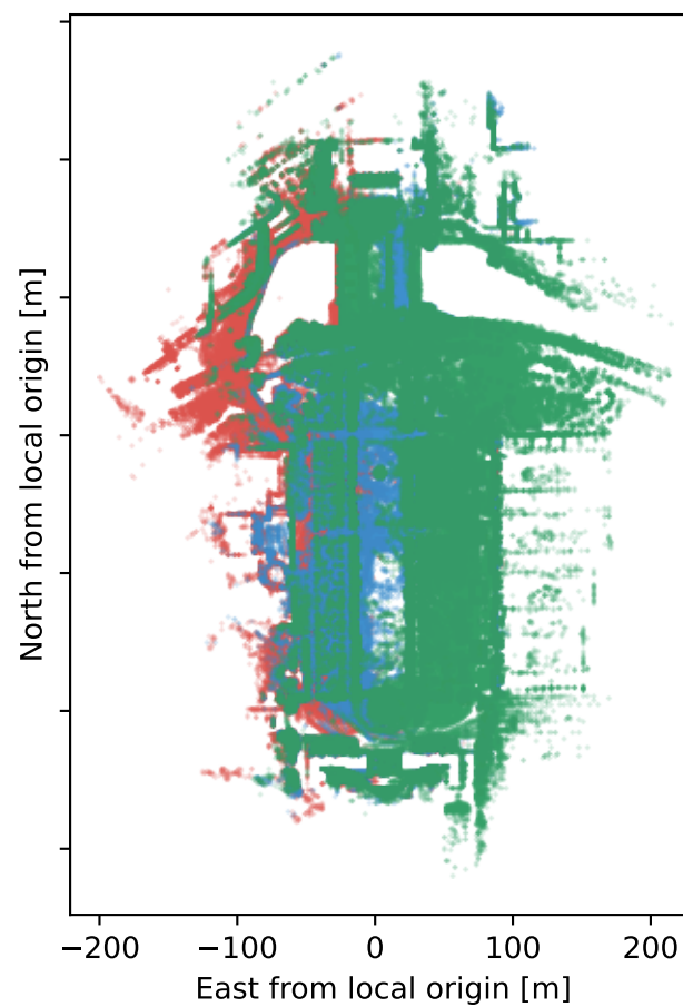
Pose + live GICP factors
