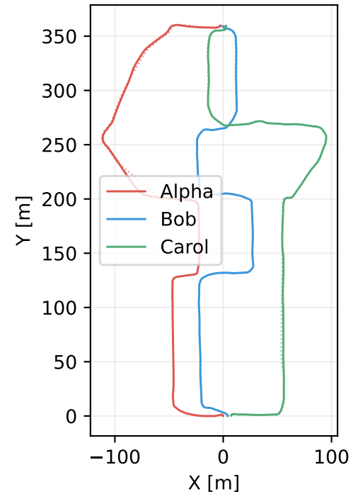
Our raw BEV + PGO Alpha + Bob + Carol · ATE 1.1446 m
