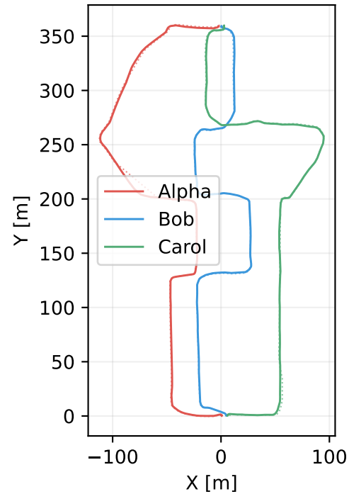
Our ellipsoid BEV + PGO Alpha + Bob + Carol · ATE 1.2682 m
