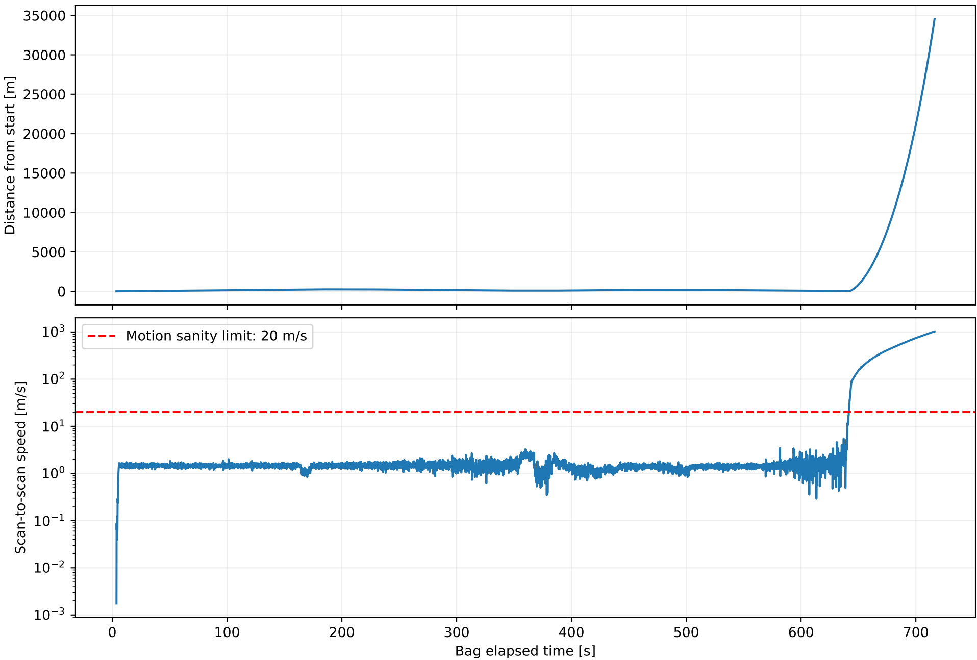
S3E_Campus_Road_1 · Alpha EllipseLIO divergence before Swarm-SLAM
