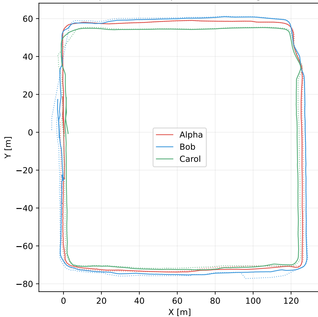
Raw EllipseLIO — independent robot alignments
