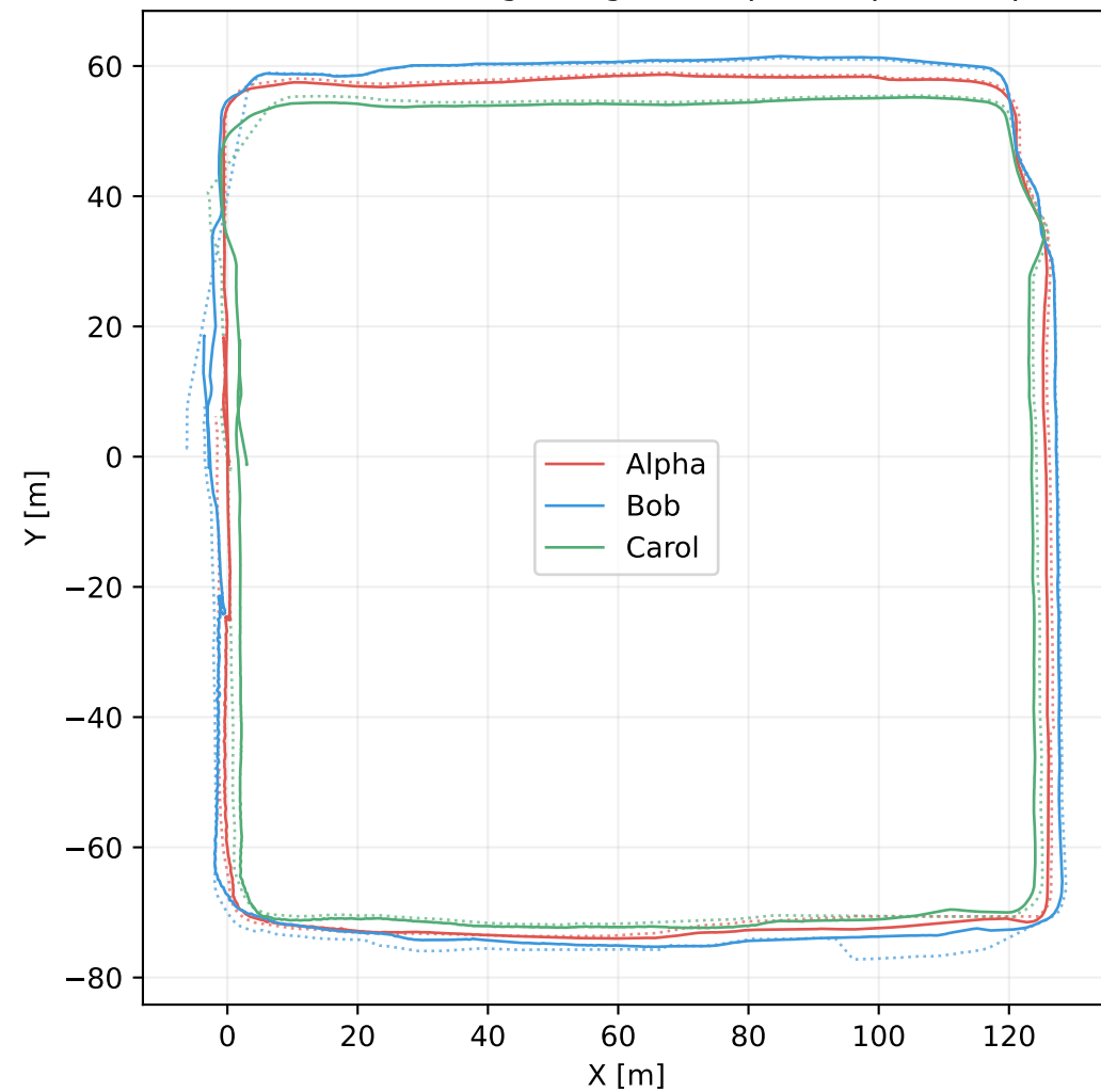
Swarm-SLAM — one rigid alignment per output component
