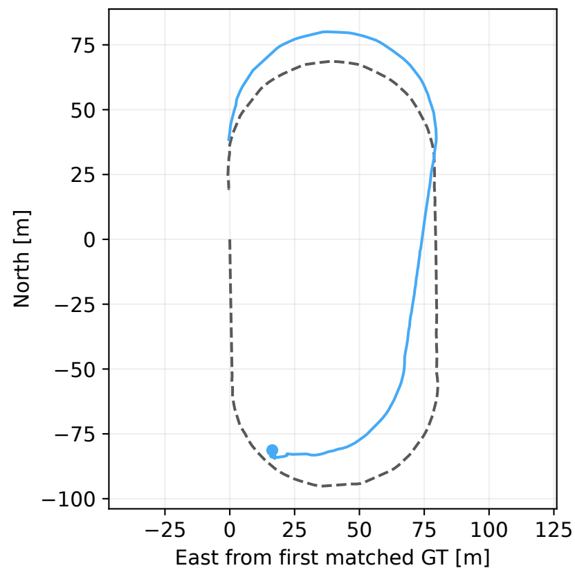
Bob: raw odometry evo ATE RMSE 25.942 m
