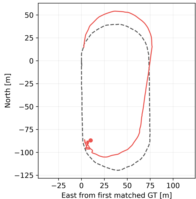
Alpha: raw odometry evo ATE RMSE 28.746 m
