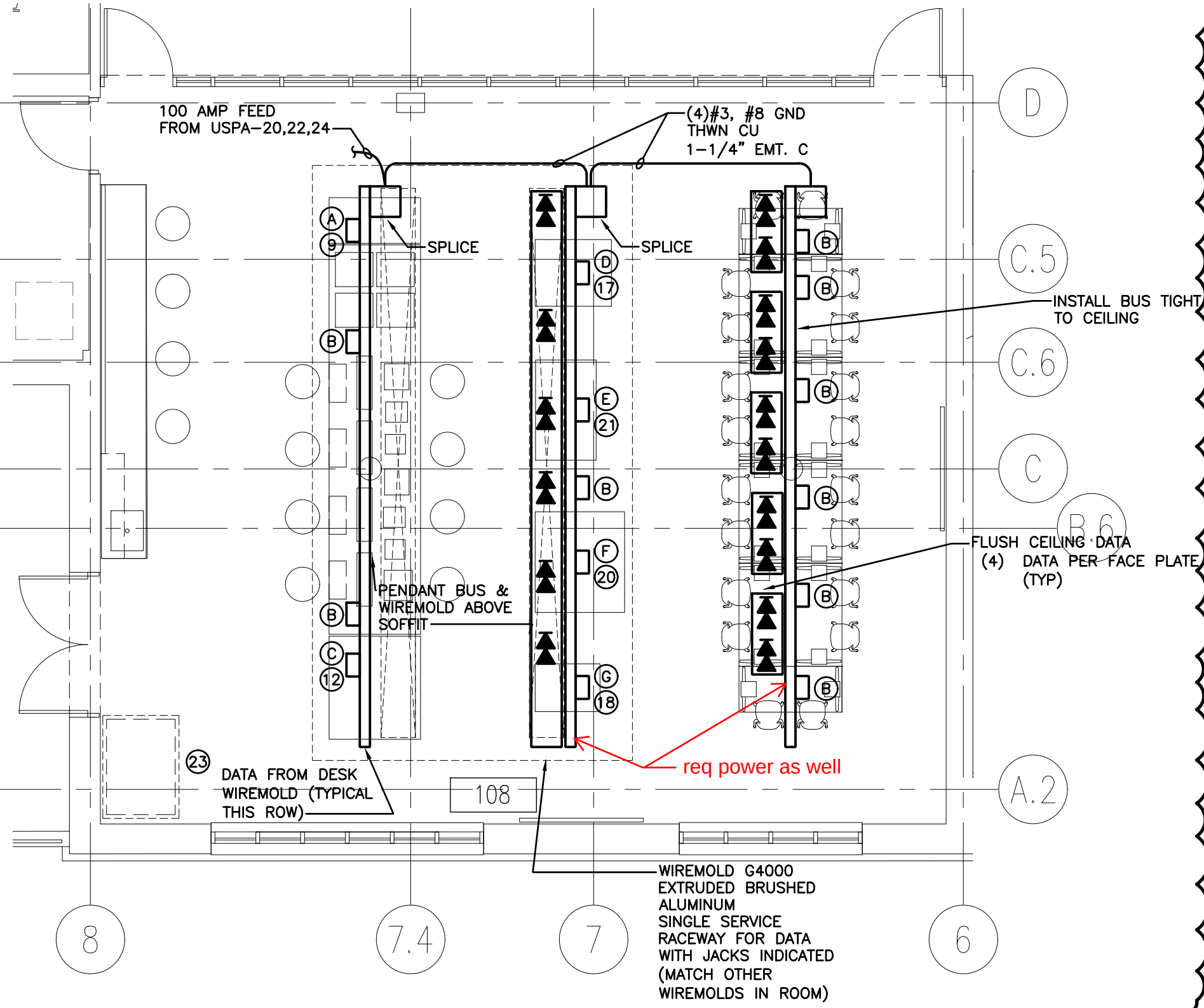
2 INNOVATION LAB OVERHEAD BUS DETAIL NORTH SCALE: 3/16" = 1'-0"
