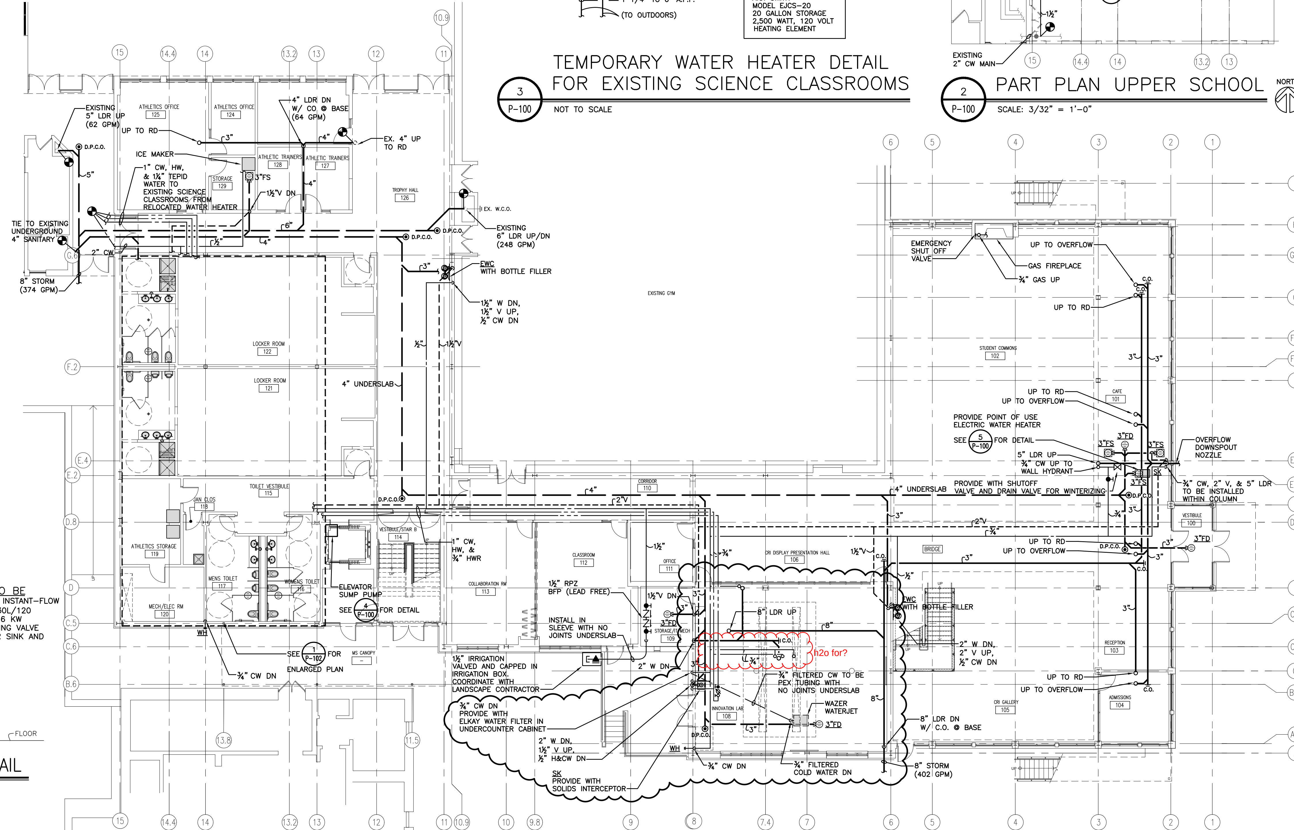
1 FIRST FLOOR PLAN-PLUMBING P-100 SCALE: 3/32" = 1'-0"
