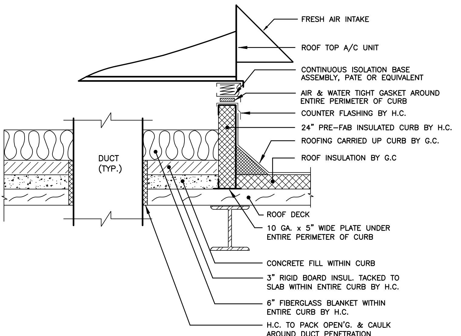
3 ROOF-TOP A/C UNIT-CURB DETAIL H-107 NOT TO SCALE
