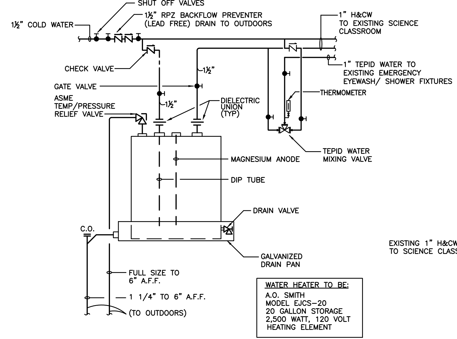
3 TEMPORARY WATER HEATER DETAIL FOR EXISTING SCIENCE CLASSROOMS P-100 NOT TO SCALE
