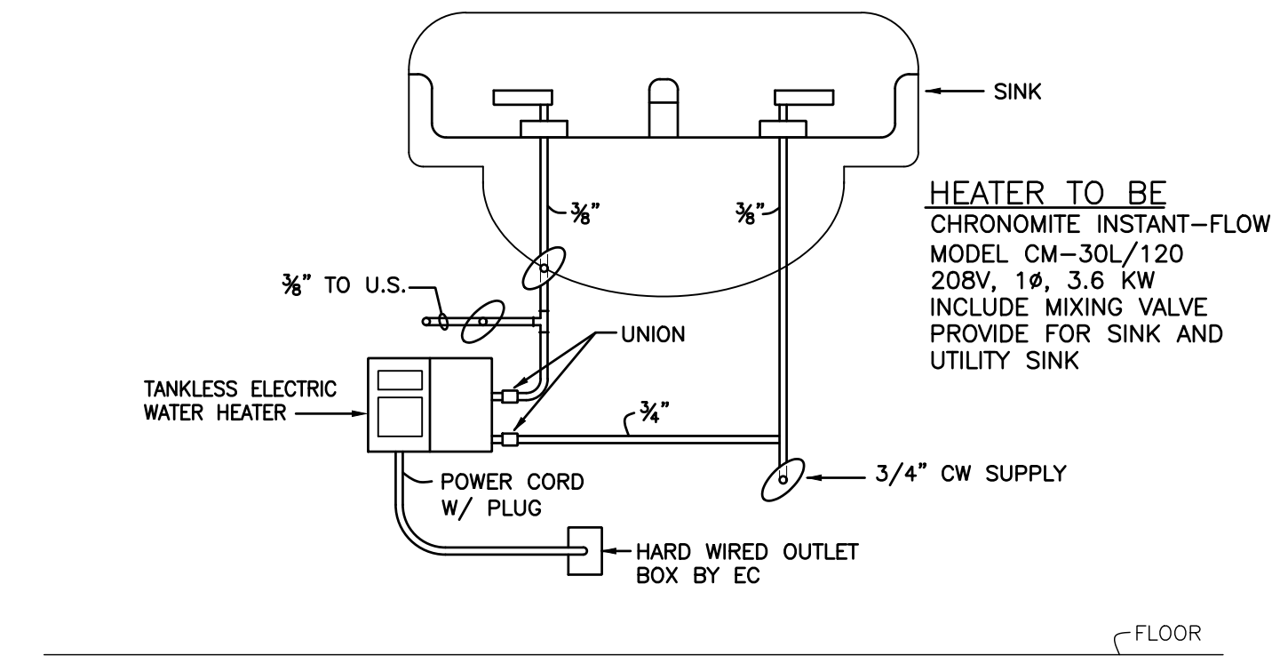
5 POINT OF USE WATER HEATER DETAIL P-100 NOT TO SCALE
