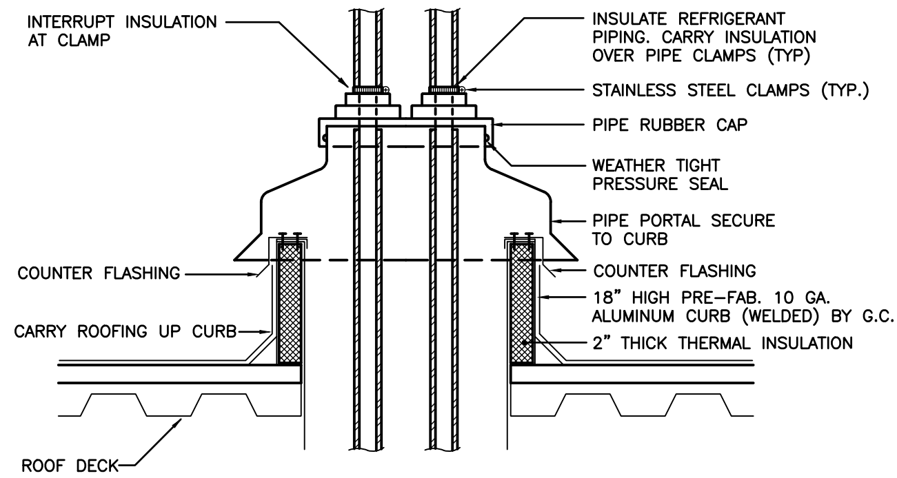
4 REFRIG. PIPING THROUGH ROOF DETAIL H-107 NOT TO SCALE
