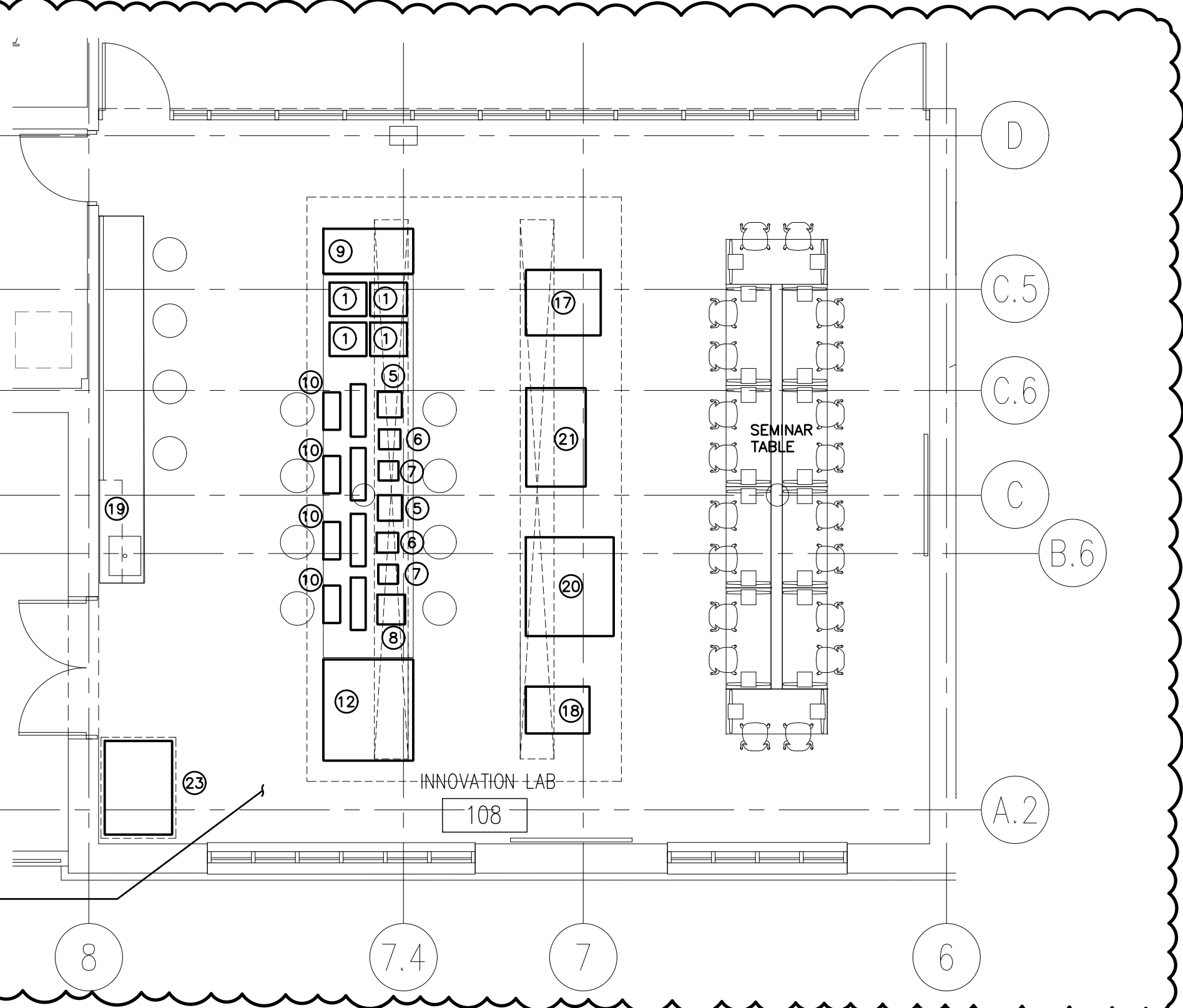
1 INNOVATION LAB EQUIPMENT PLAN - POWER NORTH SCALE: 3/16" = 1'-0"
