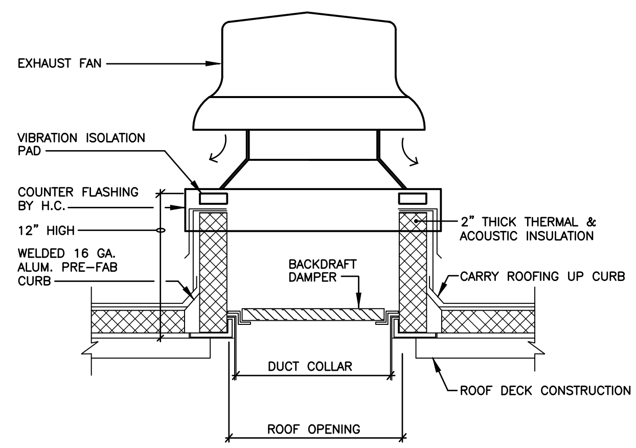
2 ROOF EXHAUST FAN DETAIL H-107 NOT TO SCALE
