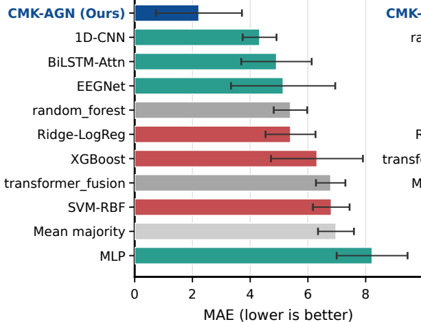
(a) FMA-UE
