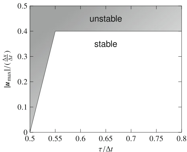
Fig. 4.5 Stability regions of |\mathbf{u}_{\max}|/(\frac{\Delta \mathbf{x}}{\Delta t}) vs. \tau/\Delta t (simplified version of Fig. 2 in [62])
