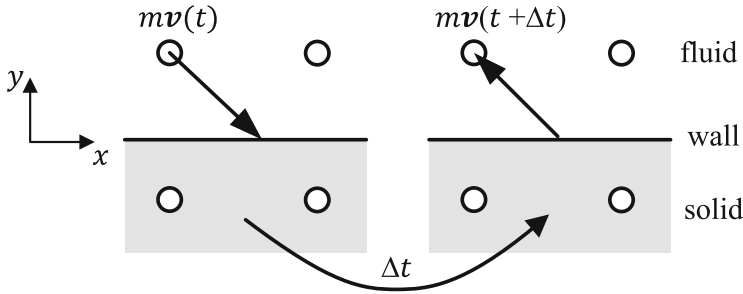
Fig. 5.10 Sketch of a moving particle with mass m and velocity \mathbf{v} hitting a rigid wall. During the collision process both normal and tangential momentum components are reversed. The average particle momentum, before and after collision, is \langle m\mathbf{v} \rangle = (m\mathbf{v}(t) + m\mathbf{v}(t + \Delta t))/2 = \mathbf{0} since \mathbf{v}(t + \Delta t) = -\mathbf{v}(t)
