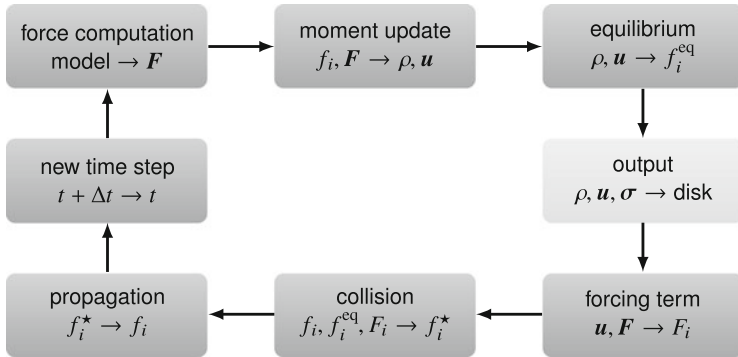
Fig. 6.1 An overview of one cycle of the LB algorithm, considering forces but not boundary conditions. The light grey box shows the optional output sub-step
