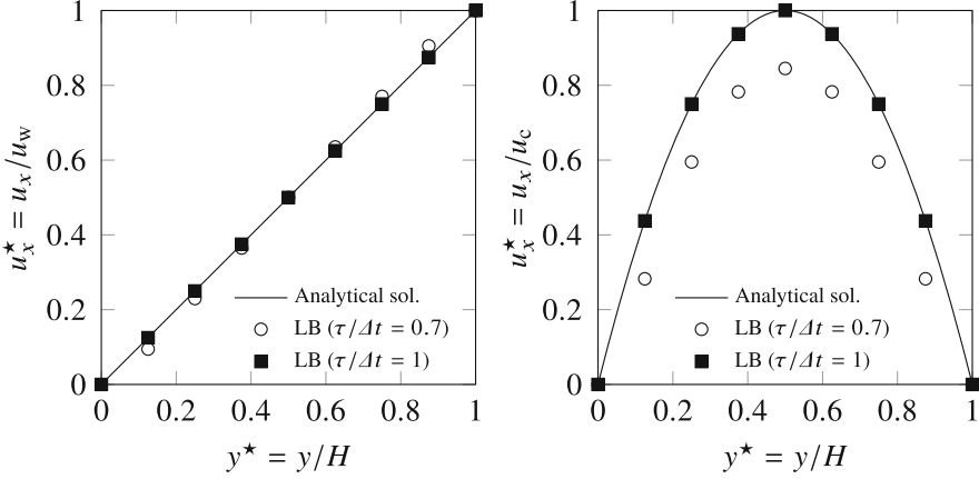
Fig. 5.23 LB solutions using the equilibrium boundary scheme for channel width N = 9 . Left plot: Couette flow; right plot: Poiseuille flow. Results with \tau/\Delta t = 0.7 are inaccurate while \tau/\Delta t = 1 leads to machine-accurate solutions
