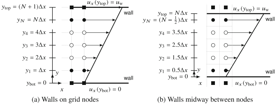
Fig. 5.14 Couette flow geometry assuming: (a) grid nodes on cell vertexes, and (b) grid nodes on cell centres. Fluid nodes: ( open circle symbol), boundary nodes: ( solid circle symbol) and solid node: ( filled squares symbol)
