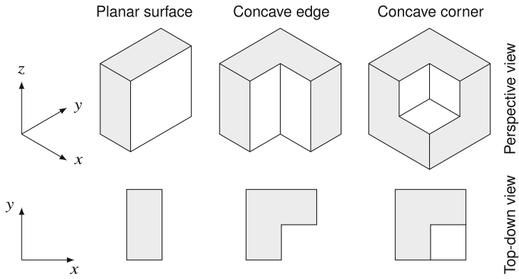
Fig. 5.30 Schematic representation of different geometrical features in 2D and 3D problems, inspired by [34]. White surfaces represent fluid-solid boundaries while grey surfaces represent cuts through the solid. The 3D plane degenerates to a 2D edge, and the two other 3D configurations degenerate to 2D corners
