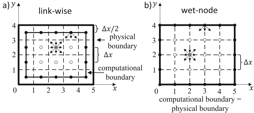
Fig. 5.7 Two discretisations of the same domain with (a) link-wise and (b) wet-node boundary conditions. Fluid nodes are illustrated as open circles (○), boundary nodes as solid circles (●)
