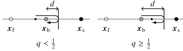
Fig. 11.5 Interpolated bounce-back cases. For q < \frac{1}{2} (left), the distance d between the wall (vertical line) and the boundary node at \mathbf{x}_b is smaller than half a lattice spacing. Interpolations are required to construct the post-collision population (small black circle). For q \geq \frac{1}{2} (right), d is larger than half a lattice spacing and the endpoint of the streaming population (small black circle) lies between the wall and \mathbf{x}_b . \mathbf{x}_s denotes a solid node behind the wall, and \mathbf{x}_f is a fluid node required for the interpolation
