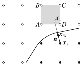
Fig. 11.9 Image-based ghost method. For each ghost node \mathbf{x}_s , the closest wall point \mathbf{x}_w is computed. The corresponding image point \mathbf{x}_i in the fluid ( open circles ) is constructed along the normal vector \mathbf{n} . Fluid properties at the image point are obtained from an interpolation in the grey region (fluid nodes A, B, C, D ). A different interpolation is required if not all interpolation support points are located within the fluid
