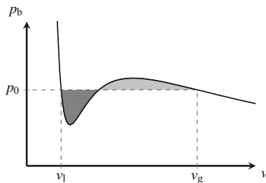
Fig. 9.2 Maxwell area construction rule for the van-der-Waals equation of state for a fixed temperature T . Note that the phase transition occurs at a pressure p_0 that equalises the areas below (dark grey) and above (light grey) the pressure curve
