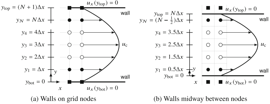
Fig. 5.17 Poiseuille flow geometry assuming: (a) grid nodes on cell vertices, and (b) grid nodes on cell centres. Fluid nodes: (open circle symbol), boundary nodes: (solid circle symbol) and solid nodes: (filled squares symbol)
