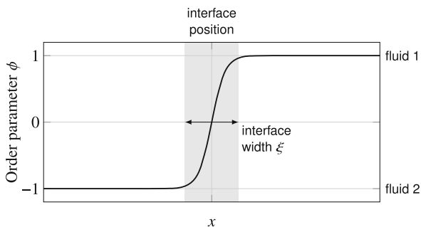
Fig. 9.4 A typical interface profile in the diffuse interface model. The order parameter varies smoothly across the interface to assume its bulk value on either side of the interface. For a multiphase system, the density varies from the gas density \rho_g to the liquid density \rho_l across the interface
