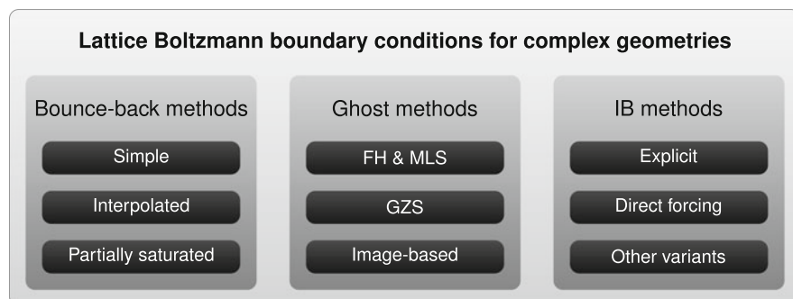
Fig. 11.2 Overview of boundary conditions for complex geometries in LB simulations as presented in this chapter. We can roughly distinguish between bounce-back, ghost and immersed-boundary (IB) methods. Each of them has several flavours. A large selection of those is covered in the following sections
