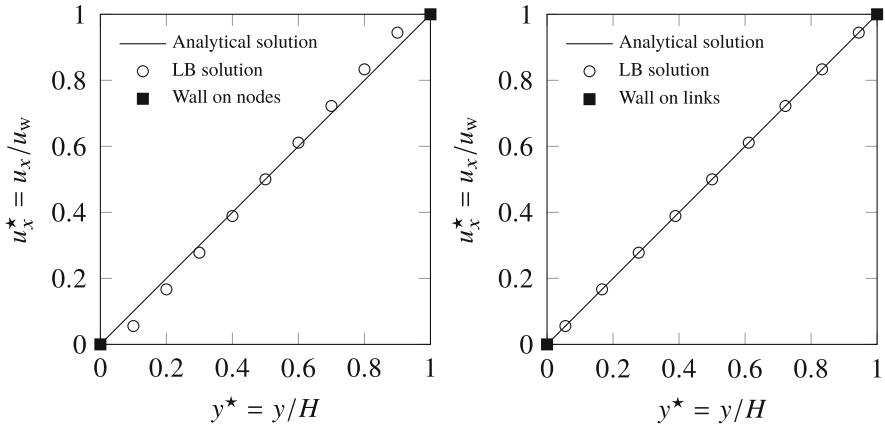
Fig. 5.15 Couette flow solution with BGK collision operator ( \tau/\Delta t = 0.9 ) and bounce-back rule ( circles ) versus analytical solution ( line ). Left panel : wall is placed on lattice nodes; right panel : wall is placed midway between lattice nodes
