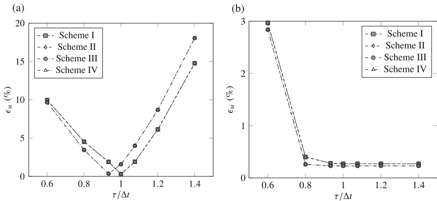
Fig. 6.2 L_2 errors for Poiseuille flow with constant force and pressure gradient, periodic conditions at inlet/outlet (LBGK, grid resolution of N_x \times N_y = 5 \times 5 , compressible equilibrium). (a) Bounce-back. (b) Non-equilibrium bounce-back
