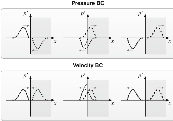
Fig. 12.4 For two different BCs, the incoming pressure pulse p'_i(c_s t - x) ( dashed ) hits a boundary at x = 0 and a reflected pulse p'_r(c_s t + x) ( dotted ) is sent back. The total pressure p'_i + p'_r ( solid ) in the physical domain ( x \leq 0 ) is also shown. (The non-physical “mirror” domain ( x > 0 ) is indicated by a darker colour)
