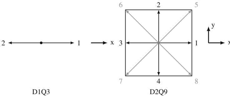
Fig. 3.3 D1Q3 and D2Q9 velocity sets. The square denoted by solid lines has an edge length 2\Delta x . Velocities with length |c_i| = 1 and \sqrt{2} are shown in black and grey, respectively. Rest velocity vectors c_0 = \mathbf{0} are not shown. See Tables 3.1, 3.2 and 3.3 for more details
