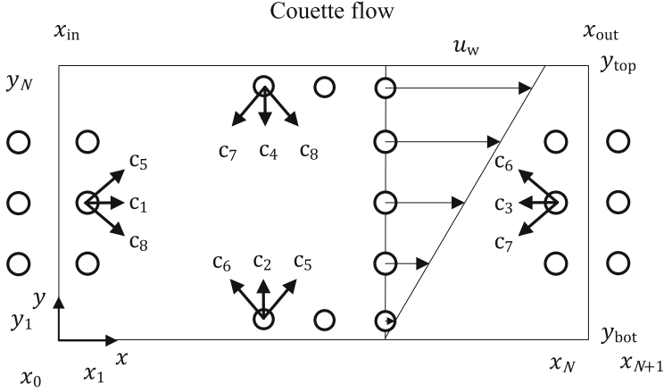
Fig. 5.13 Couette flow with unknown boundary populations annotated. The layer of wall nodes goes from x_0 to x_{N+1} , while the layer where inflow/outflow conditions are applied goes from y_1 to y_N . Corner nodes, e.g. (x_0, y_0) , belong to wall layers
