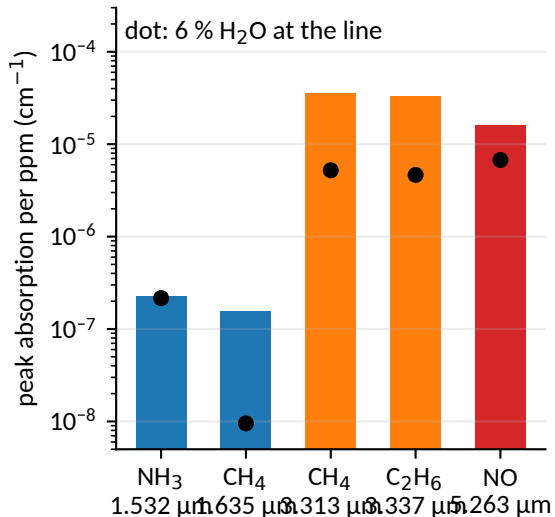
(a) HITRAN line strengths
