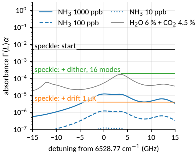
(b) NH 3 line vs speckle floor
