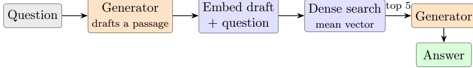
Figure 6: HyDE. The generator first writes the encyclopedia passage it imagines would answer the question; the search runs on the average of the draft’s and the question’s embeddings. The draft’s factual errors are discarded — only its vector is used.
