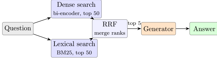
Figure 4: Hybrid retrieval. Dense and lexical rankings over the same corpus are merged by Reciprocal Rank Fusion; the BM25 row is this diagram with the dense branch removed.
