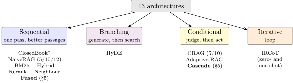
Figure 3: The compared architectures grouped by control flow. *ClosedBook retrieves nothing and serves as the floor. The two architectures in bold are introduced in Section 5.
