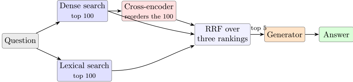
Figure 10: Fused retrieval, the cascade’s first stage. The cross-encoder is one voter among three rather than the arbiter: dense, lexical, and reranked orderings of the same candidate pool are merged by RRF (Eq. 2). A passage found by dense retrieval is voted for twice (bi-encoder rank and cross-encoder rank); a passage only the lexical index found is voted for once — the lexical list is there to rescue passages dense retrieval missed, not to outvote it.
