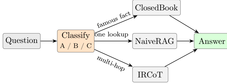
Figure 9: Adaptive-RAG (training-free form). One classification call routes each question to the no-retrieval, single-step, or iterative branch; the branches are the very architectures of the neighbouring rows.
