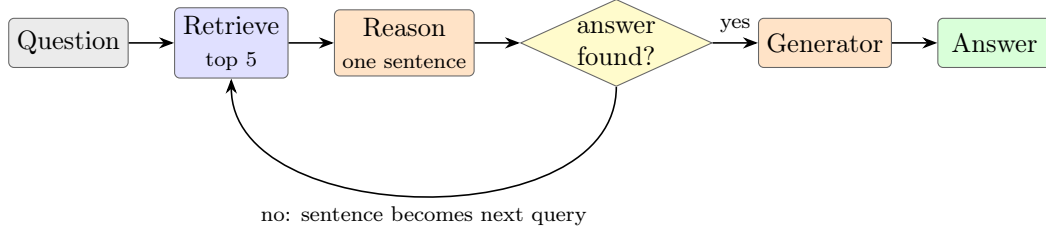
Figure 7: IRCoT. Each reasoning sentence names entities the question never mentioned, and is used verbatim as the next retrieval query; accumulated passages (up to 15) go to the same reader prompt as NaiveRAG.
