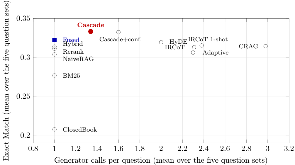
Figure 1: Answer quality against generator cost for every architecture measured in this article, averaged over the five question sets. The proposed cascade (red) reaches the highest mean Exact Match at a fraction of the cost of the iterative and corrective methods; its first stage alone (Fused, blue) already dominates the single-call architectures. Per-set results, in which no single architecture wins everywhere, are analysed in Section 7.
