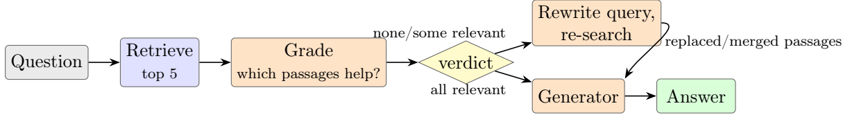
Figure 8: CRAG (offline form). The generator grades its own retrieval; on a poor grade the query is rewritten and the corpus searched again, replacing (no passage relevant) or topping up (some relevant) the context.
