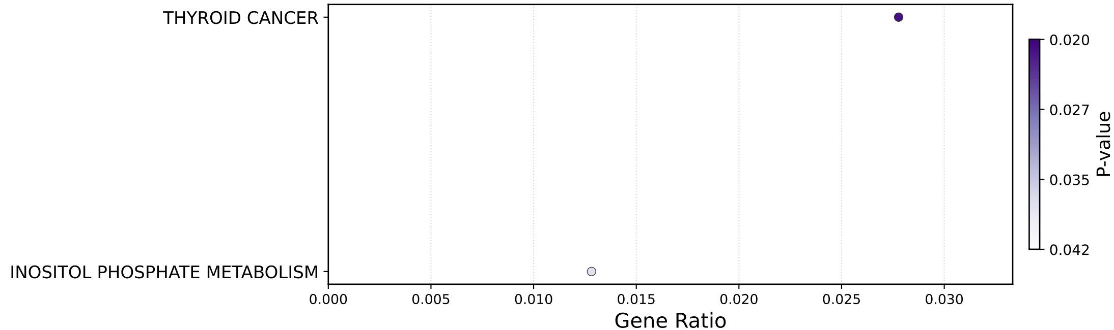
enrichment_groupA — KEGG dotplot (P-value<0.05)
