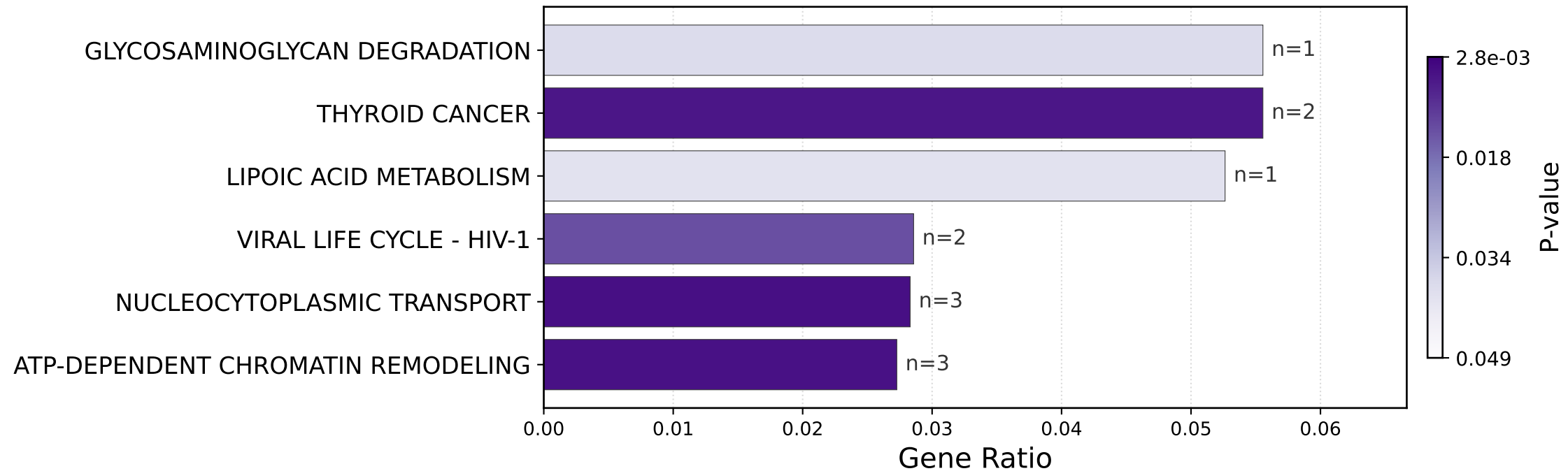
enrichment_groupB — KEGG barplot (P-value<0.05)
