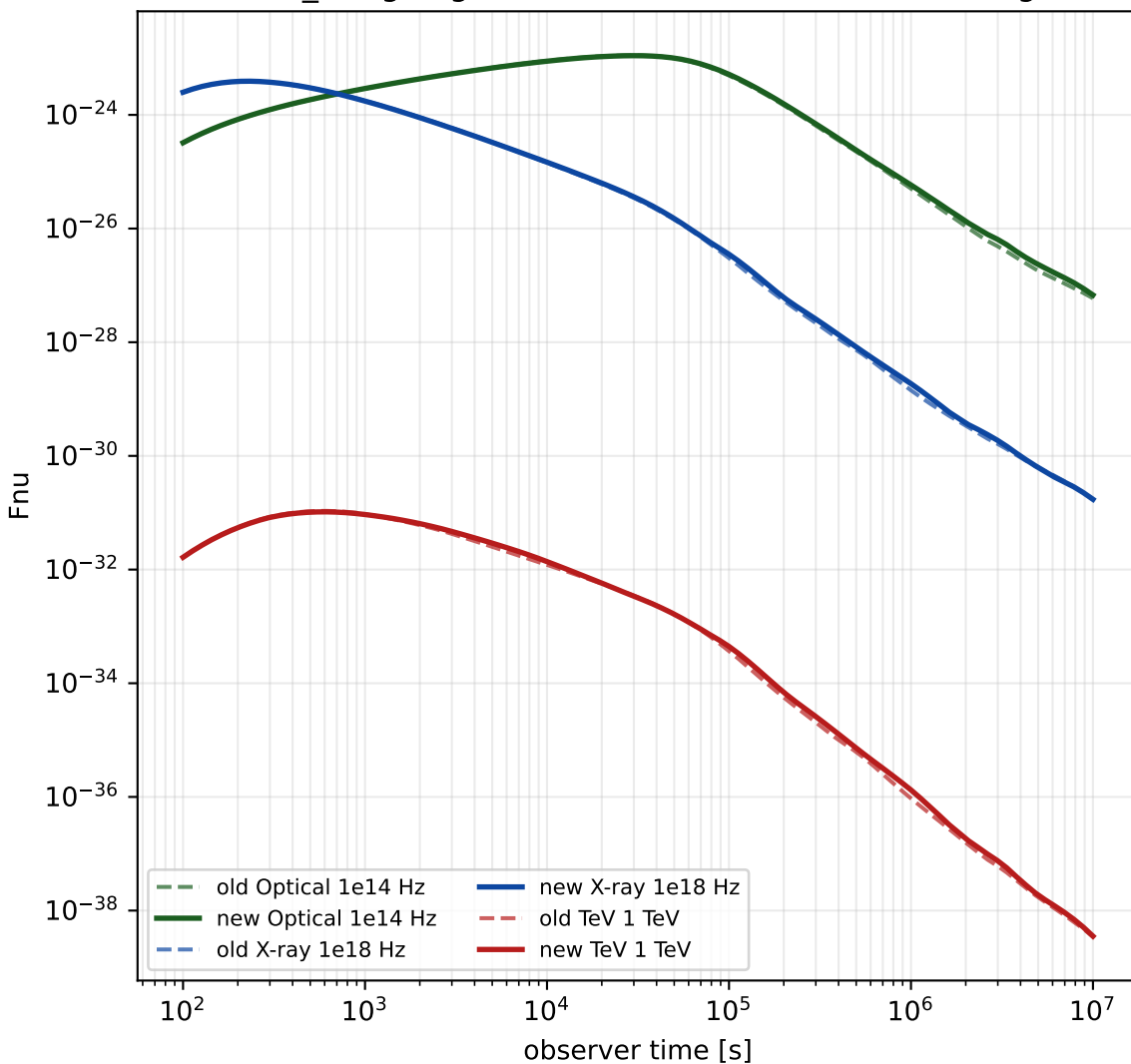
slc1_mm2 light curves: old vs new front tracking
