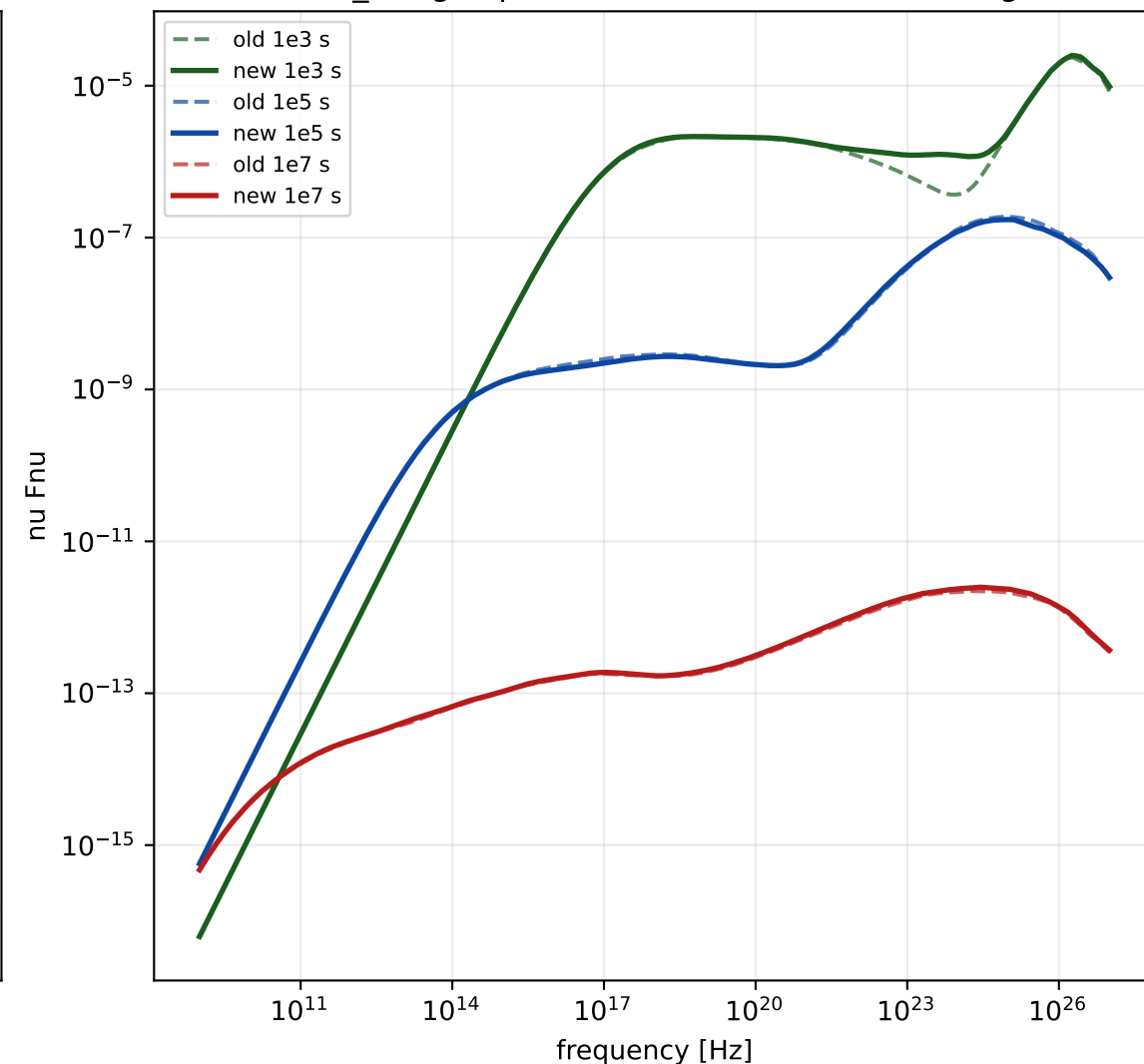
slc1_mm2 spectra: old vs new front tracking
