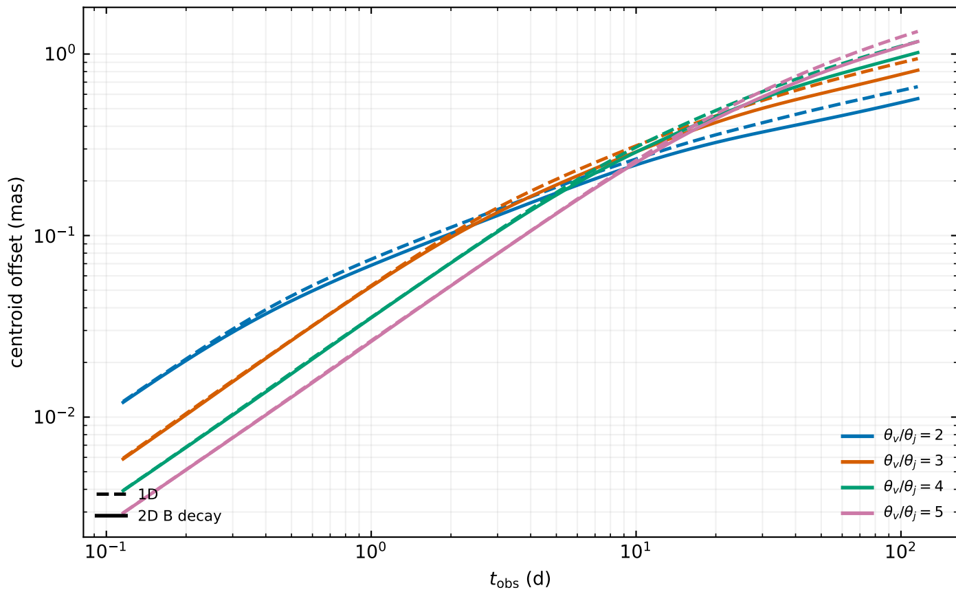
Flux-centroid offset at \nu = 1e + 10 Hz
