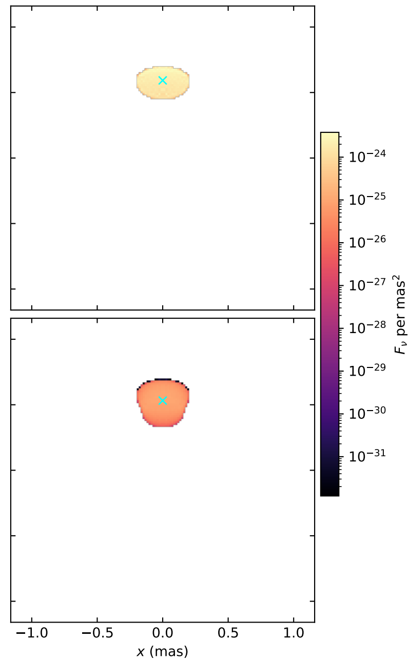
Sky maps at \nu = 1\text{e} + 10\text{ Hz} , \theta_\nu/\theta_j = 3
