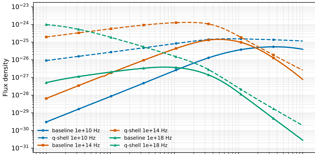
2D q-shell transport: light-curve comparison
